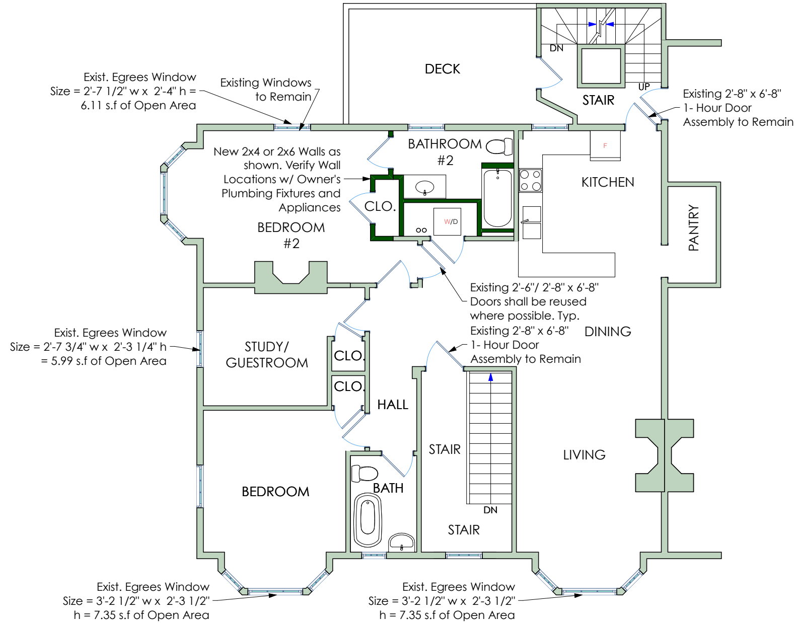
1 PROPOSED THIRD FLOOR PLAN SCALE: 1/8" = 1'-0" 0 4' 8' 16'
