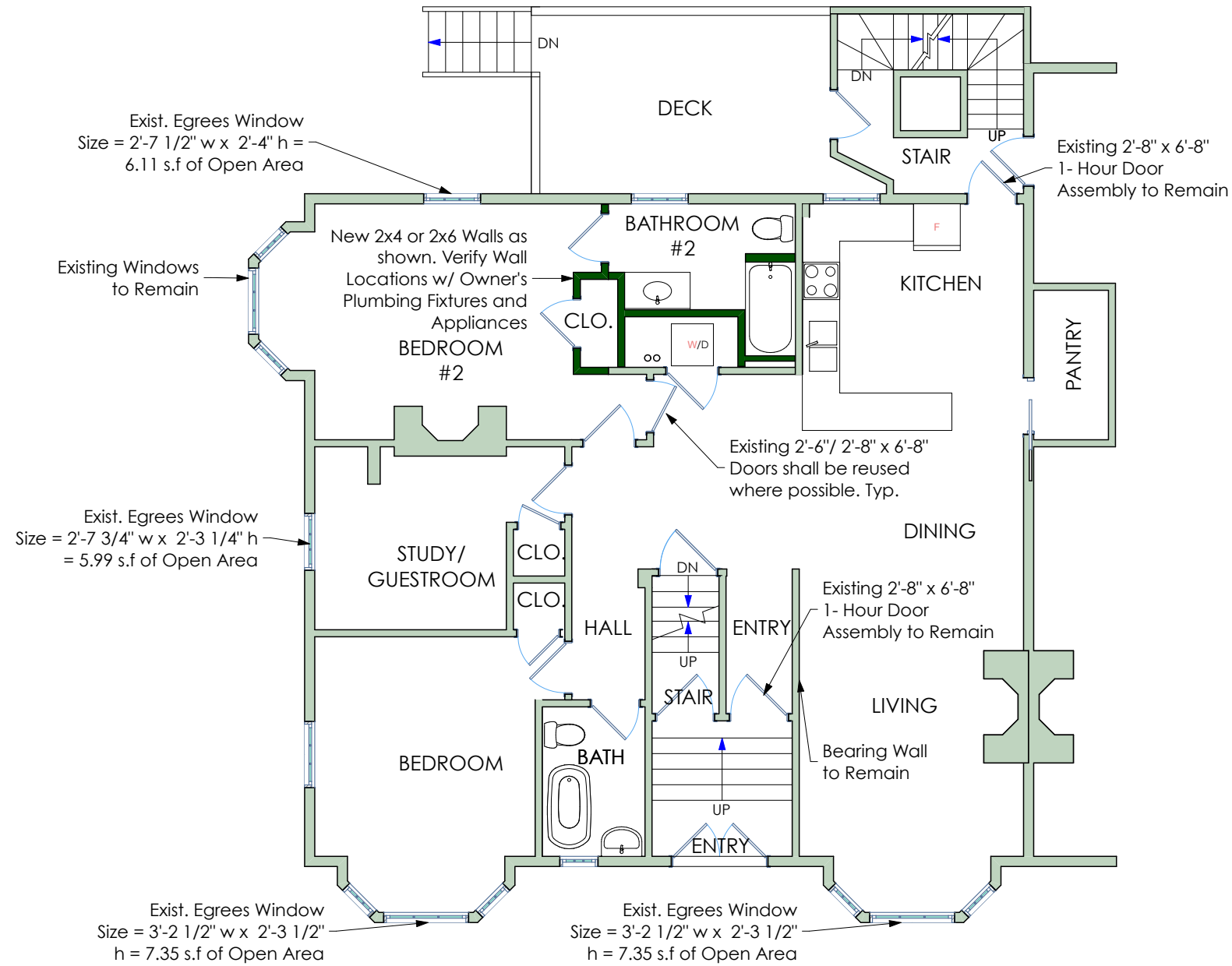
Proposed First Floor Plan SCALE: 1/8" = 1'-0"
