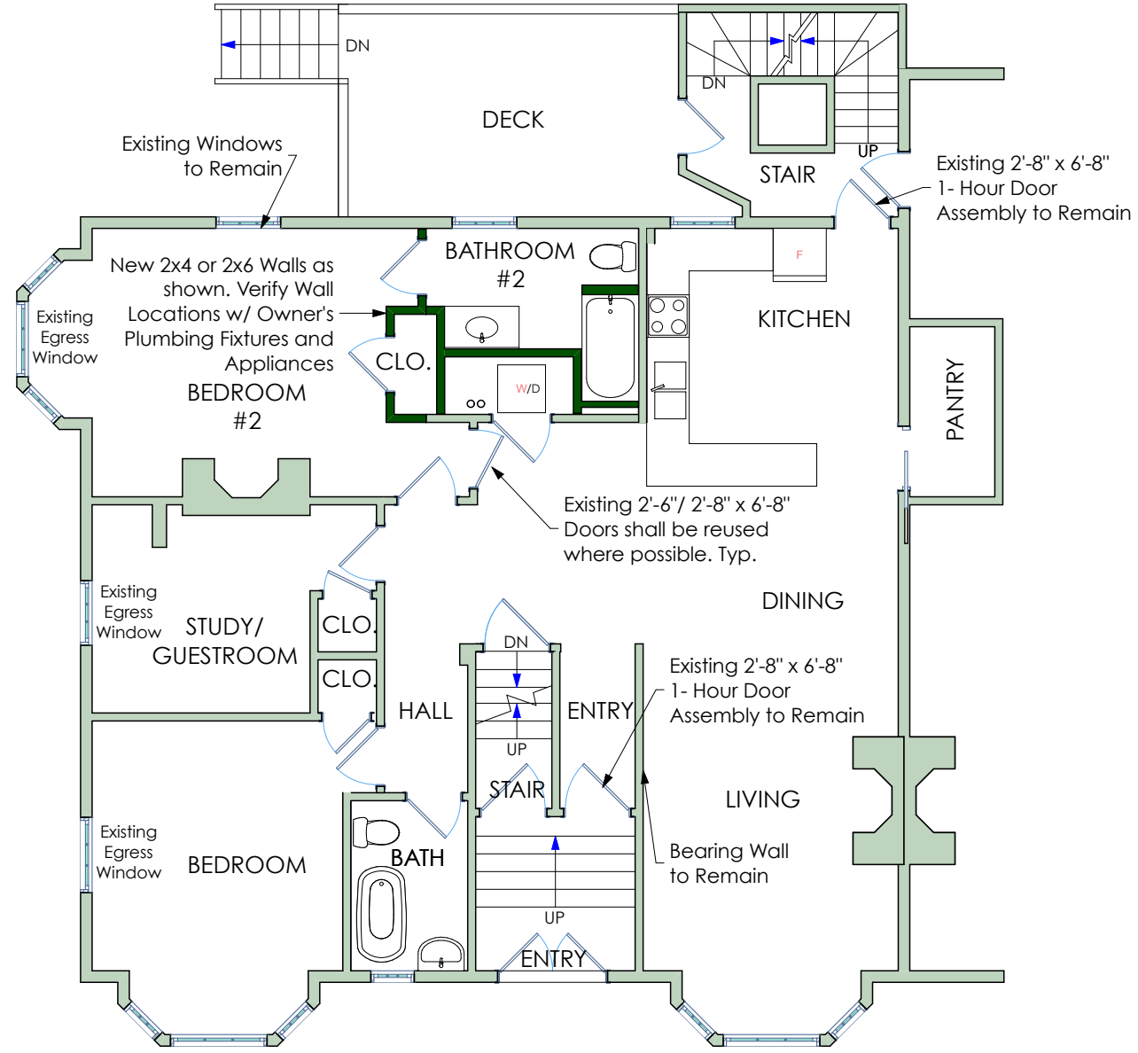
1 Proposed First Floor Plan SCALE: 1/8" = 1'-0" 0 4' 8' 16'
