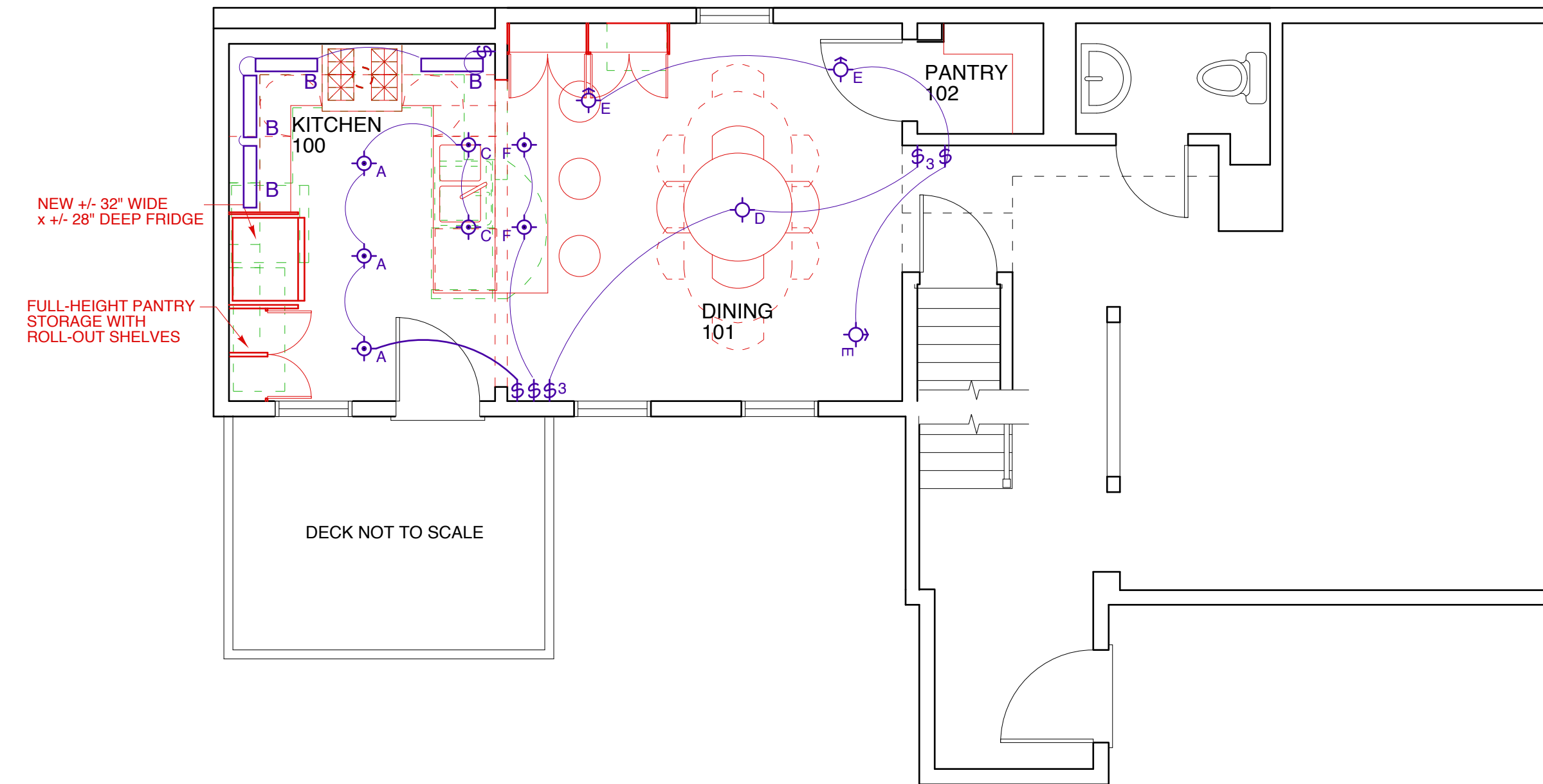
PROPOSED MAIN LEVEL
