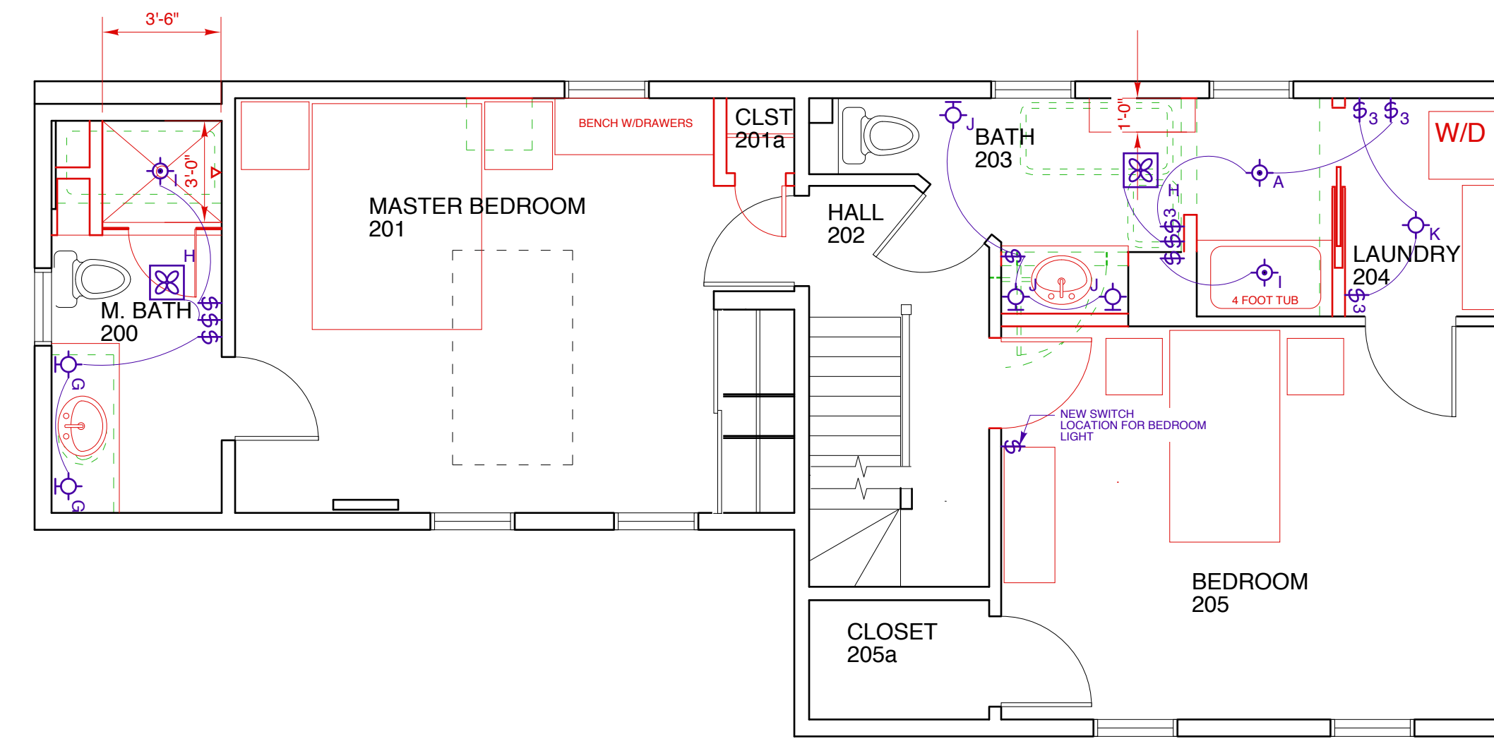
PROPOSED SECOND LEVEL
