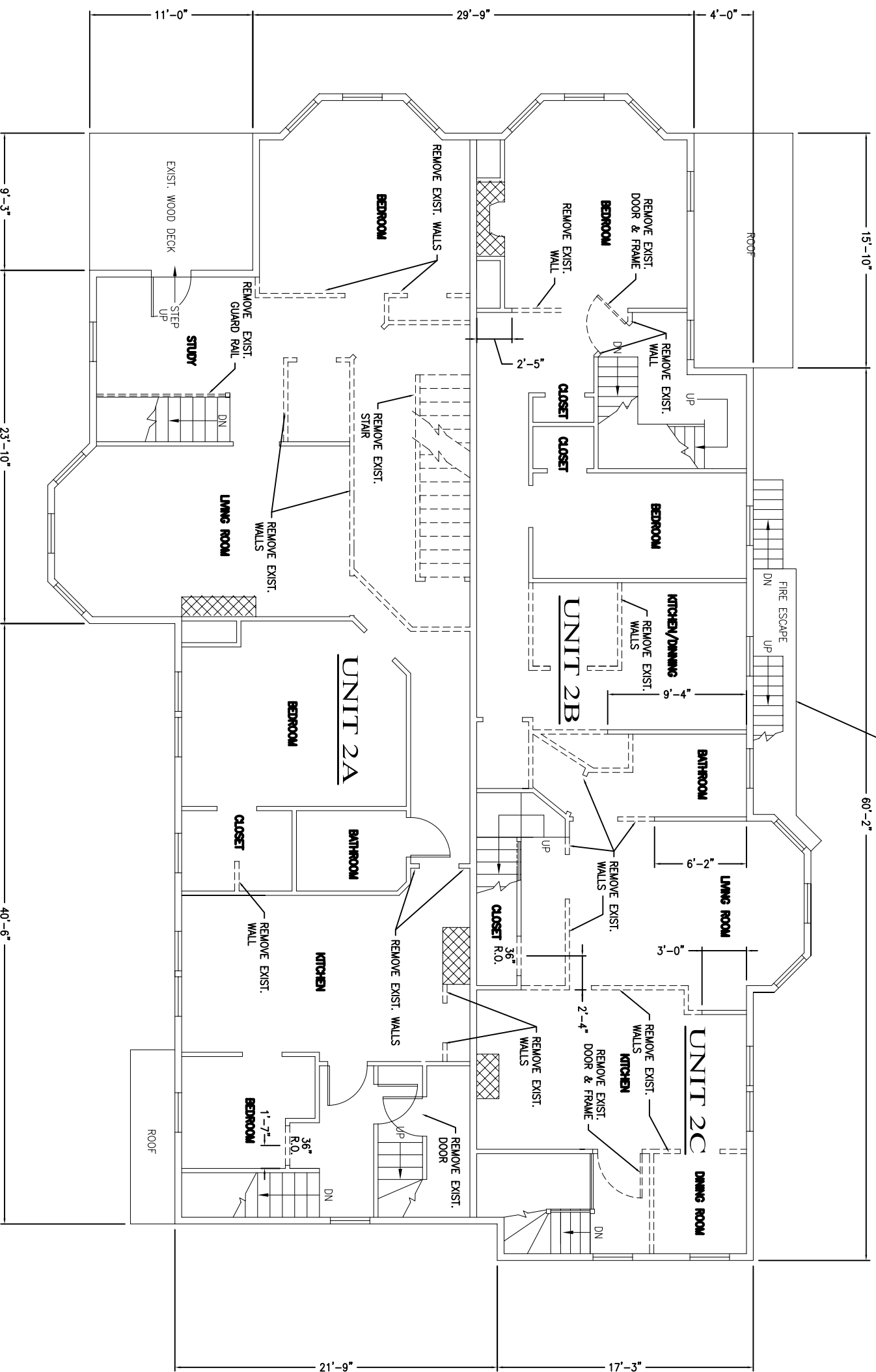
SECOND FLOOR DEMOLITION PLAN 1/4"=1'-0"
