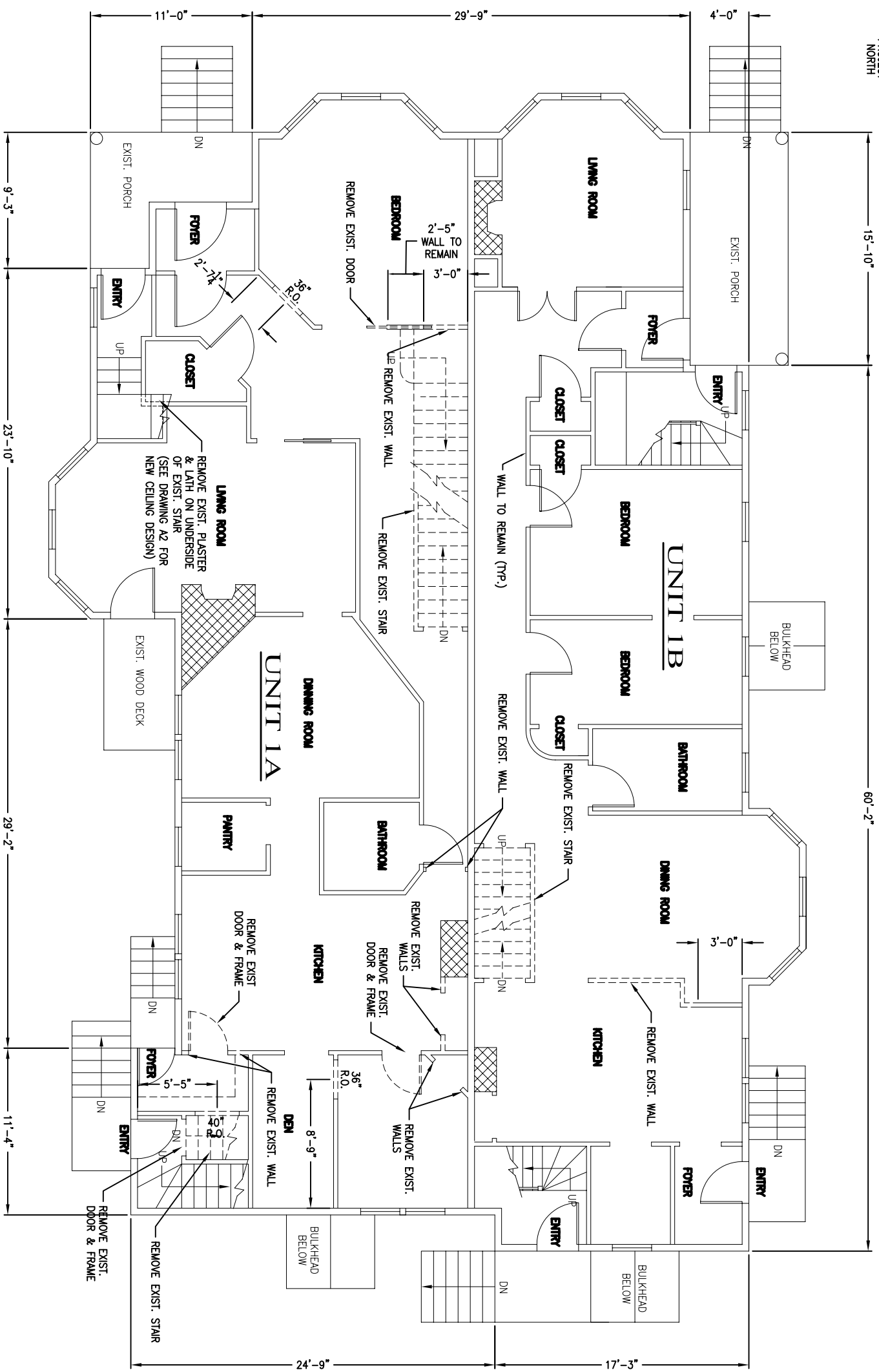
FIRST FLOOR DEMOLITION PLAN 1/4"=1'-0"
