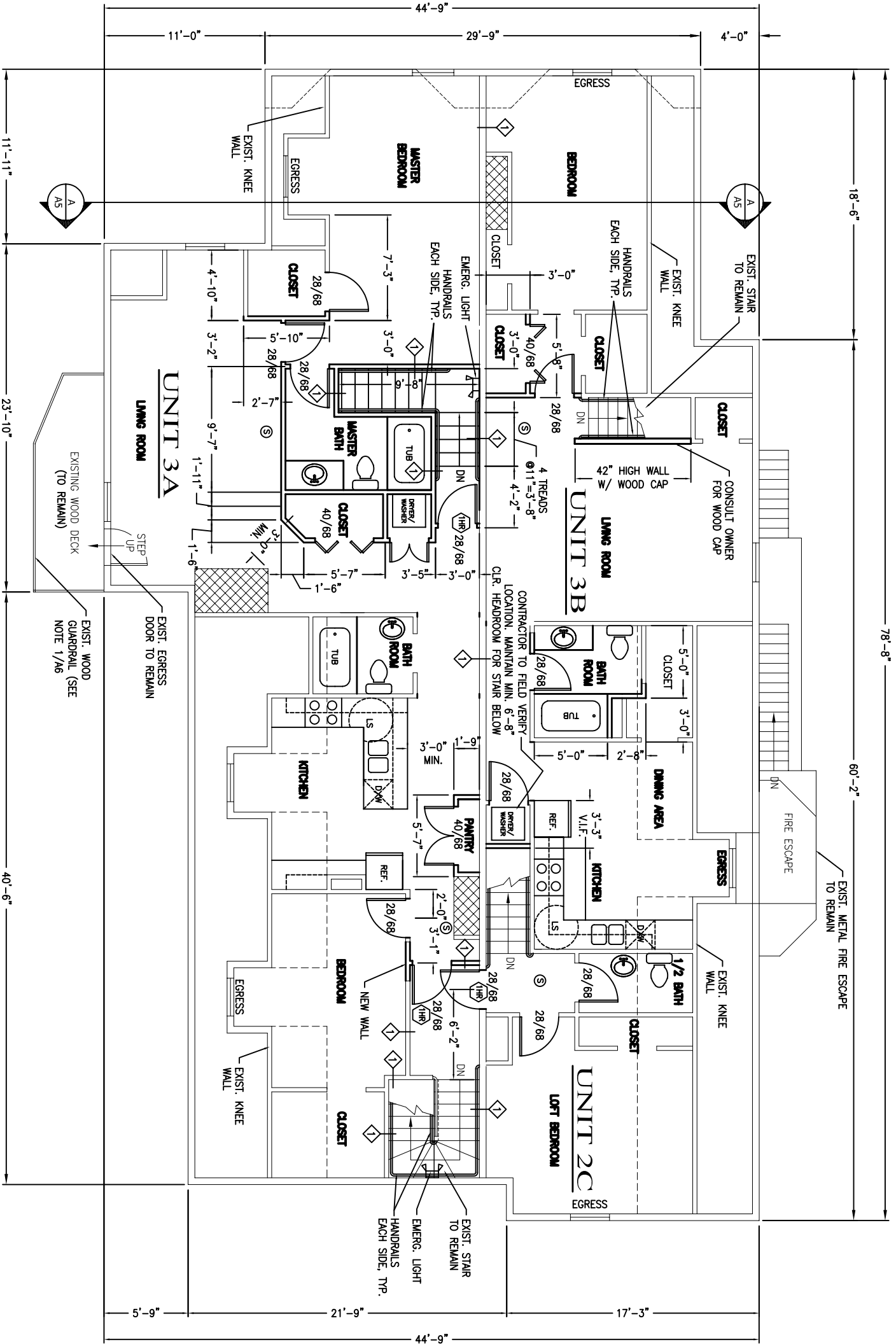
THIRD FLOOR PLAN 1/4"=1'-0"
