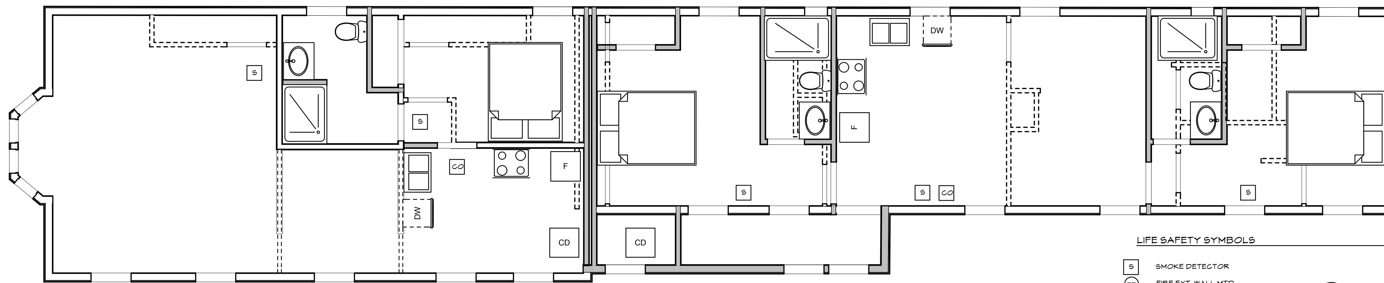
1 Second Floor Ceiling Plan A5.1 SCALE: 1/4" = 1'-0"
