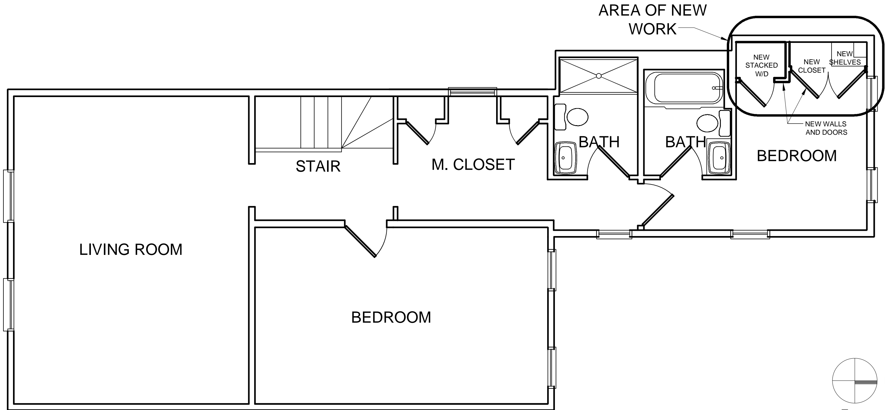
FLOOR PLAN PROPOSED LAUNDRY ROOM RENOVATIONS 19 PINE STREET, PORTLAND, ME
