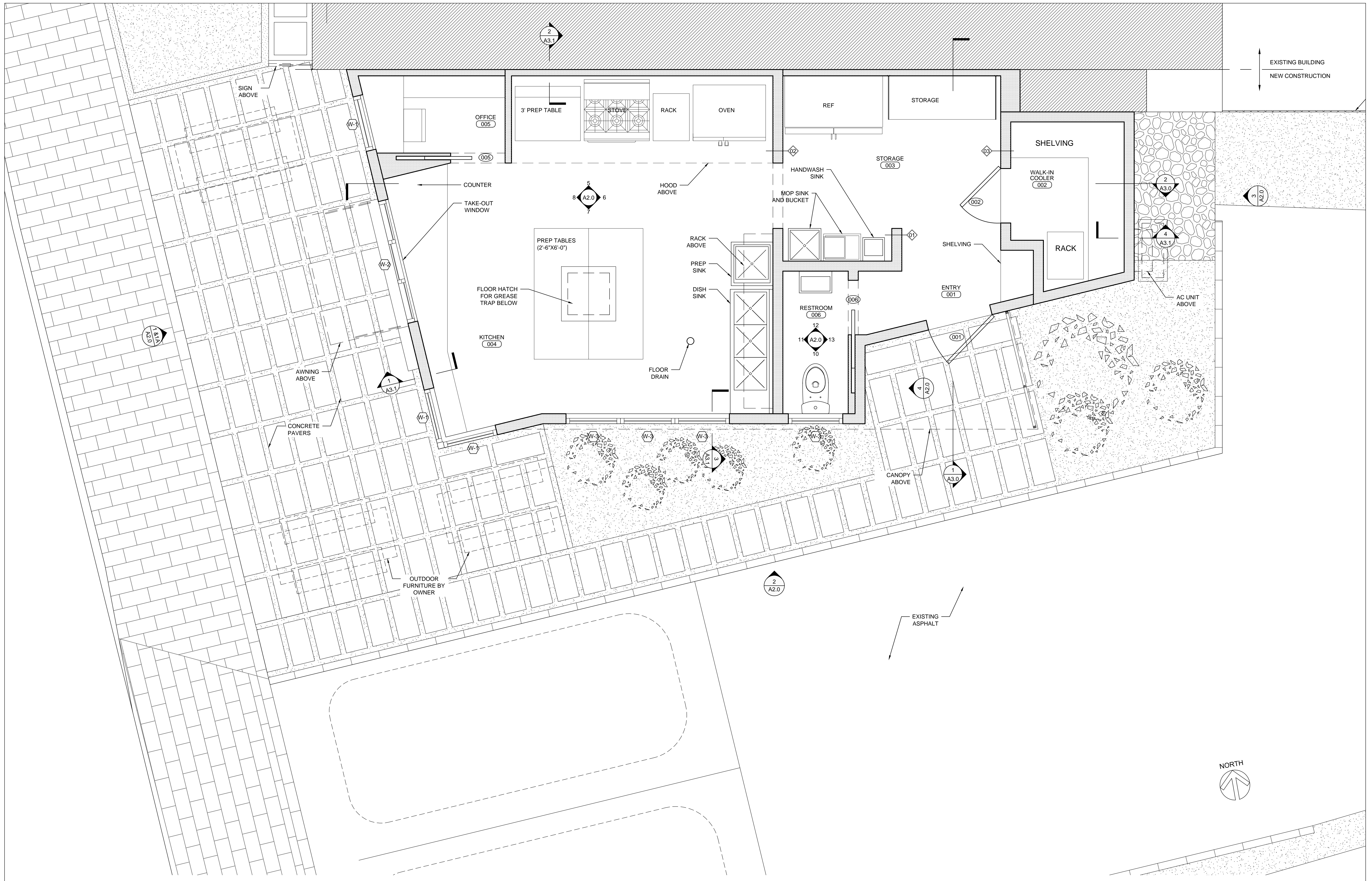
1 NEW FLOOR PLAN 1/2" = 1'-0"
