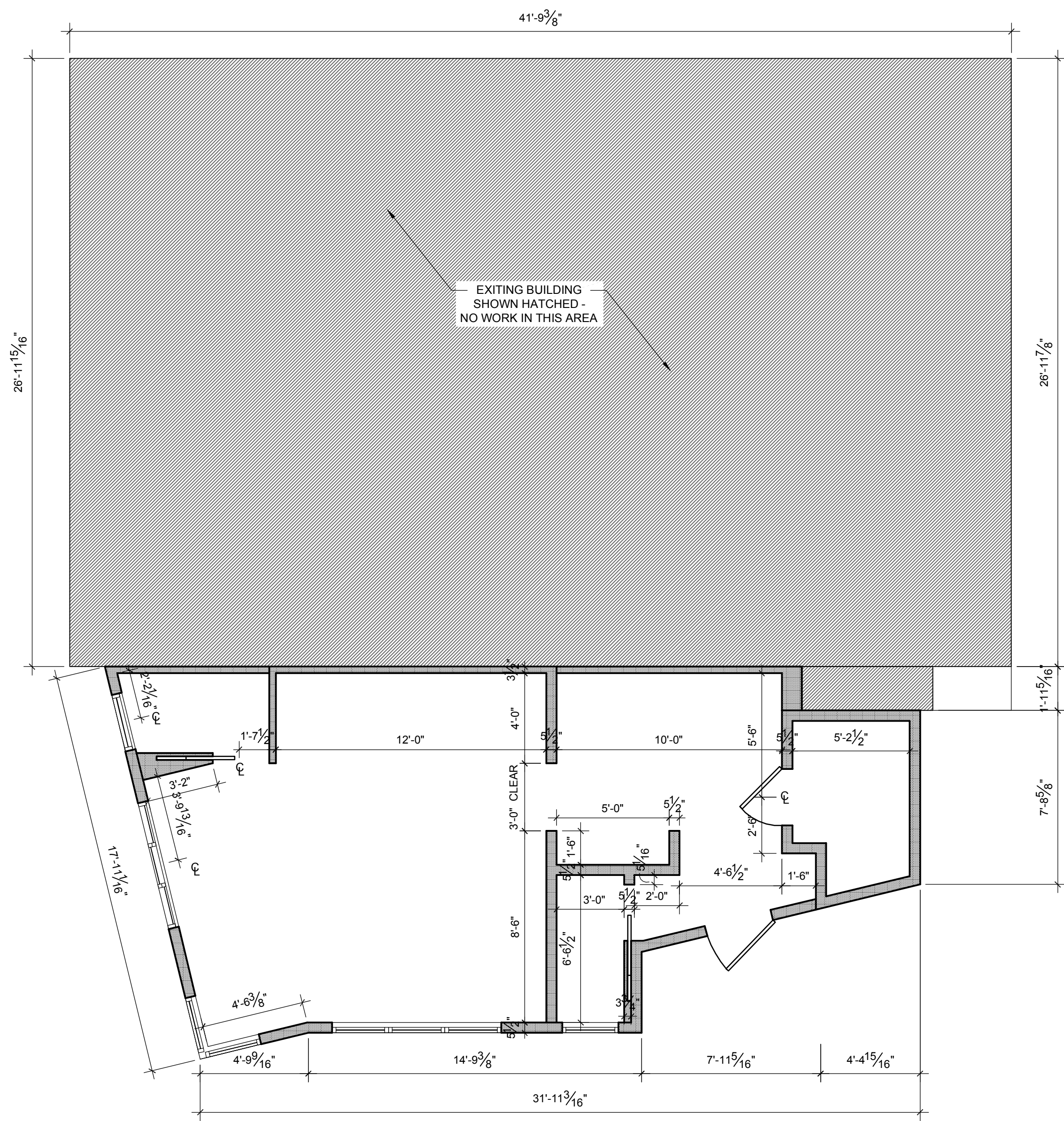
2 DIMENSIONAL FLOOR PLAN 1/4" = 1'-0"
