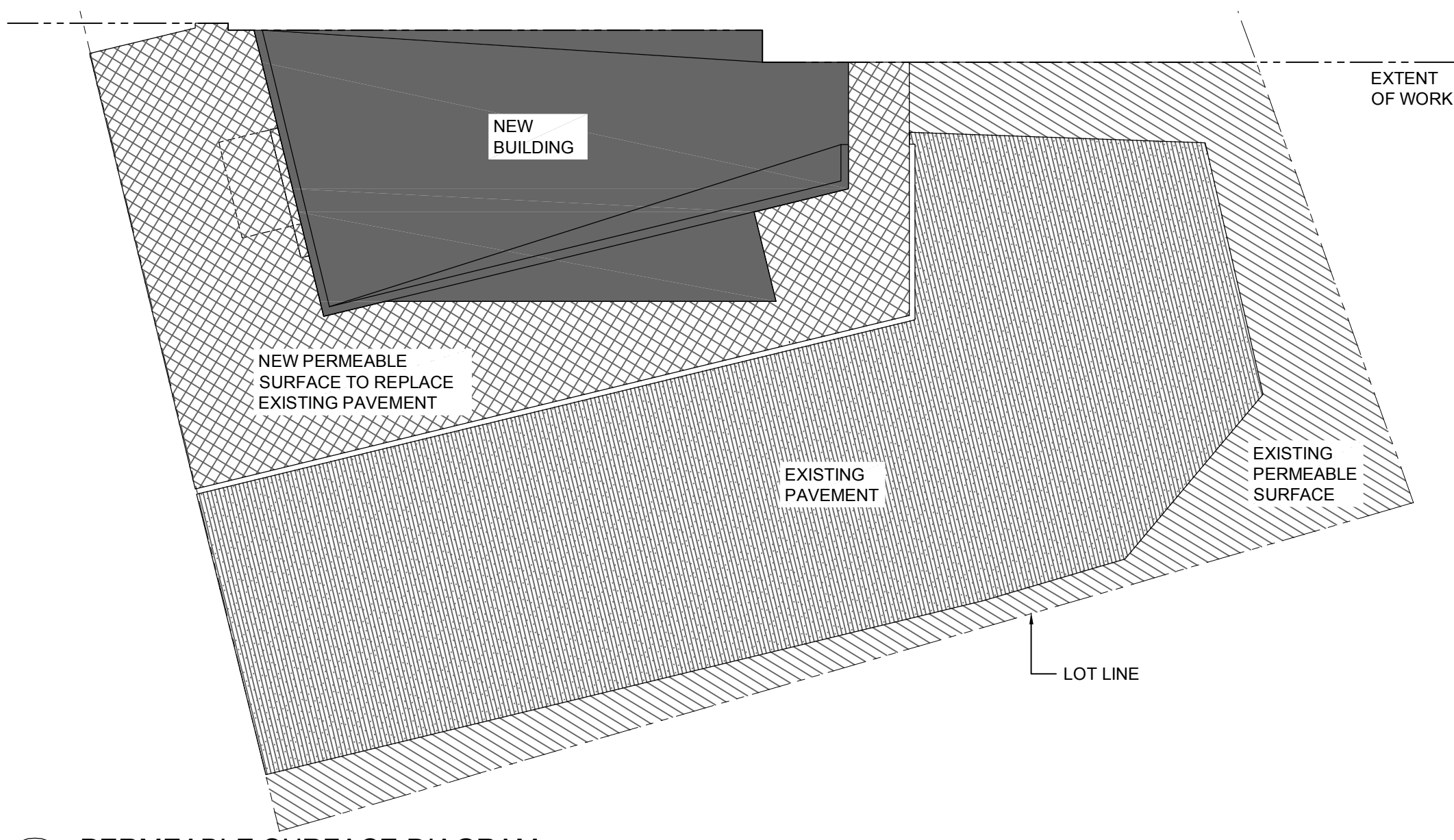
3 PERMEABLE SURFACE DIAGRAM 1/16" = 1'-0"
