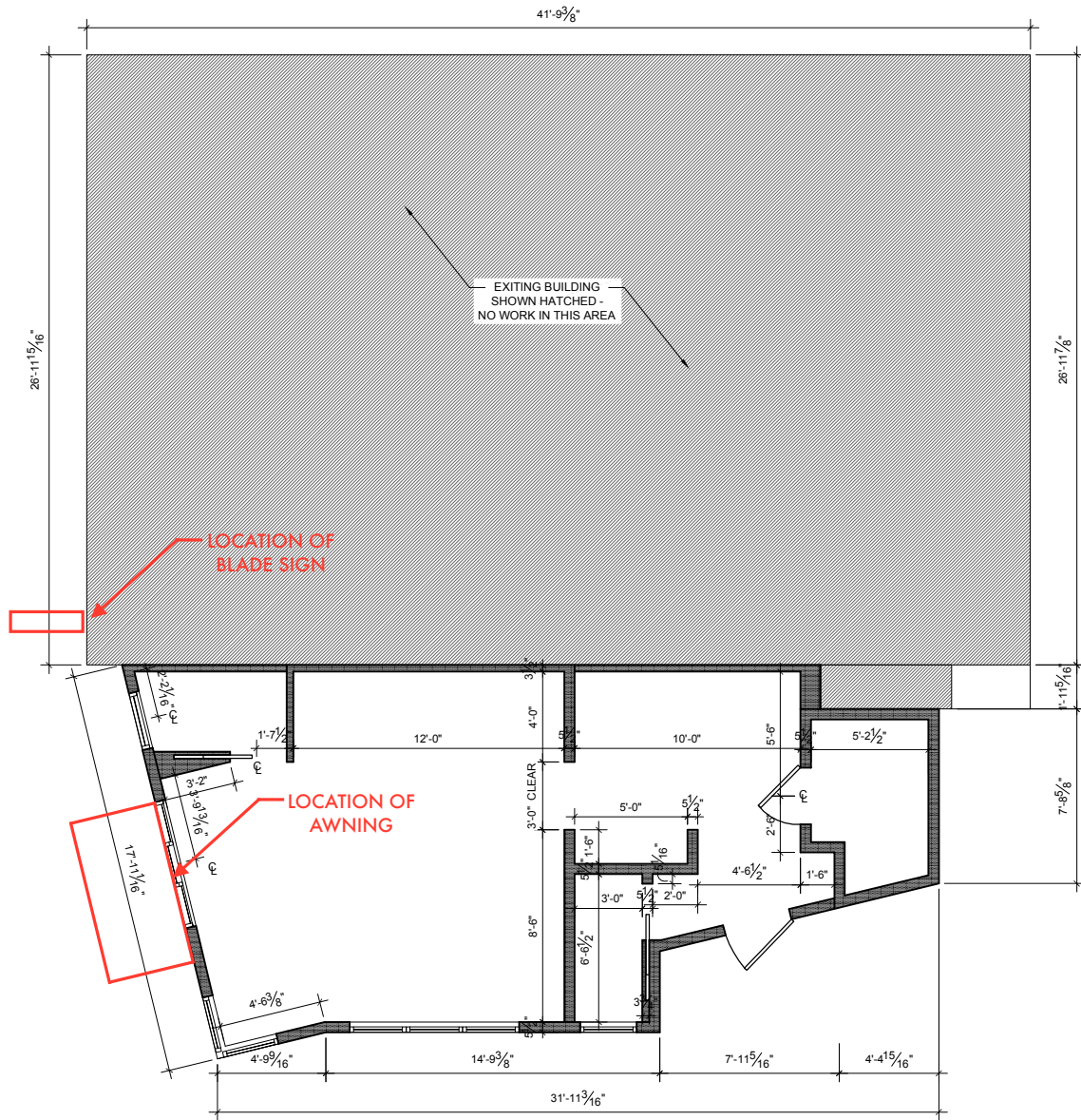
2 DIMENSIONAL FLOOR PLAN N.T.S. - FOR REFERENCE ONLY
