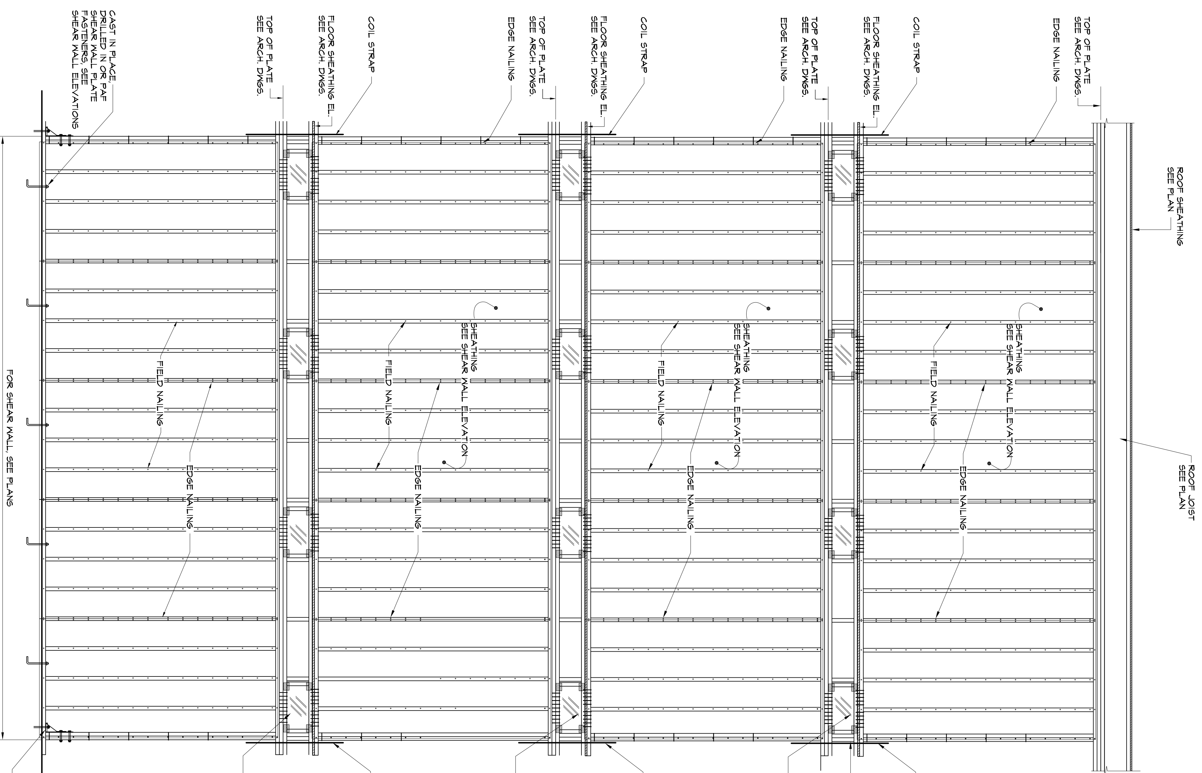
TYPICAL SHEAR WALL ELEVATION PARALLEL TO JOISTS
