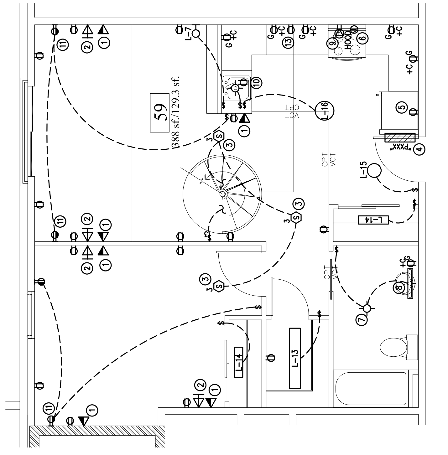
L TYPICAL UNIT TYPE "L" - (LOWER FLOOR) ELECTRICAL PLAN SCALE: 1/4"=1'-0"
