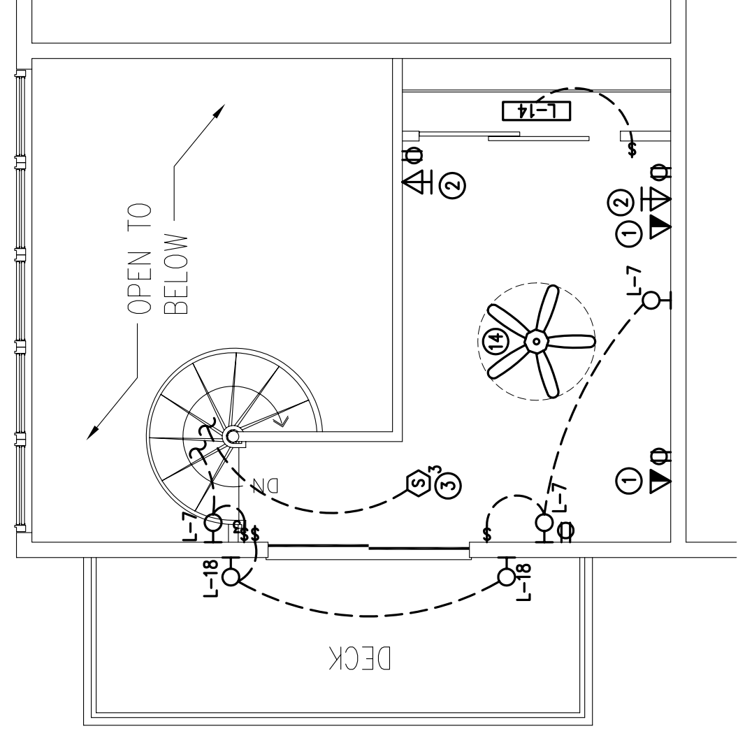
L TYPICAL UNIT TYPE "L" - (UPPER FLOOR) ELECTRICAL PLAN SCALE: 1/4"=1'-0"
