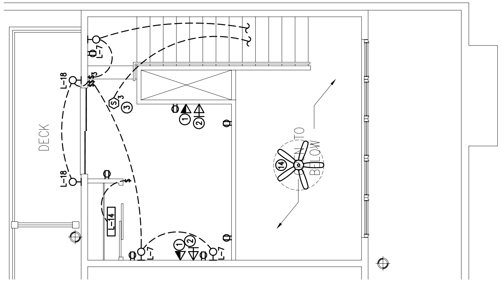
1 TYPICAL UNIT TYPE "I" - (UPPER FLOOR) ELECTRICAL PLAN SCALE: 1/4"=1'-0"
