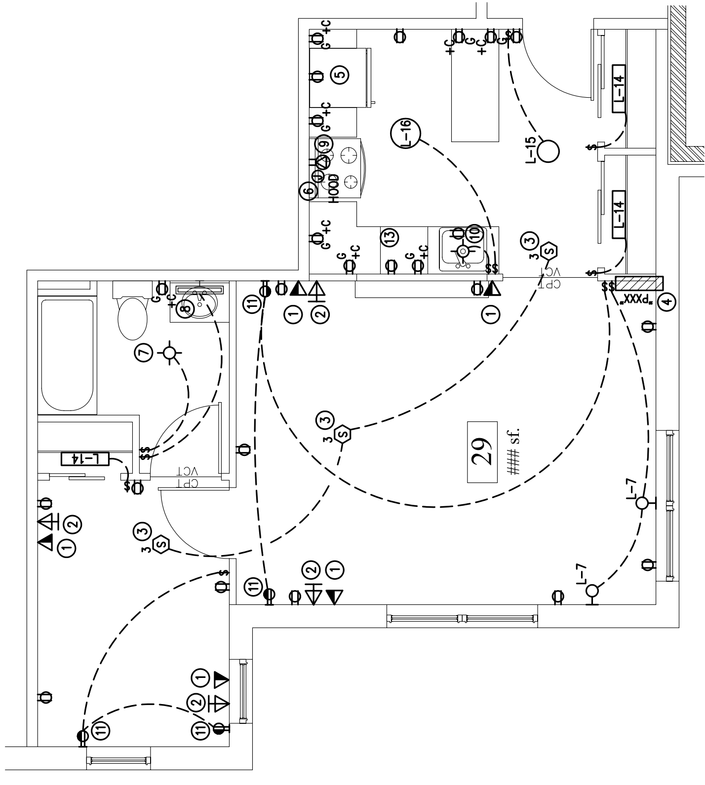
6 TYPICAL UNIT TYPE "G" - ELECTRICAL PLAN SCALE: 1/4"=1'-0"
