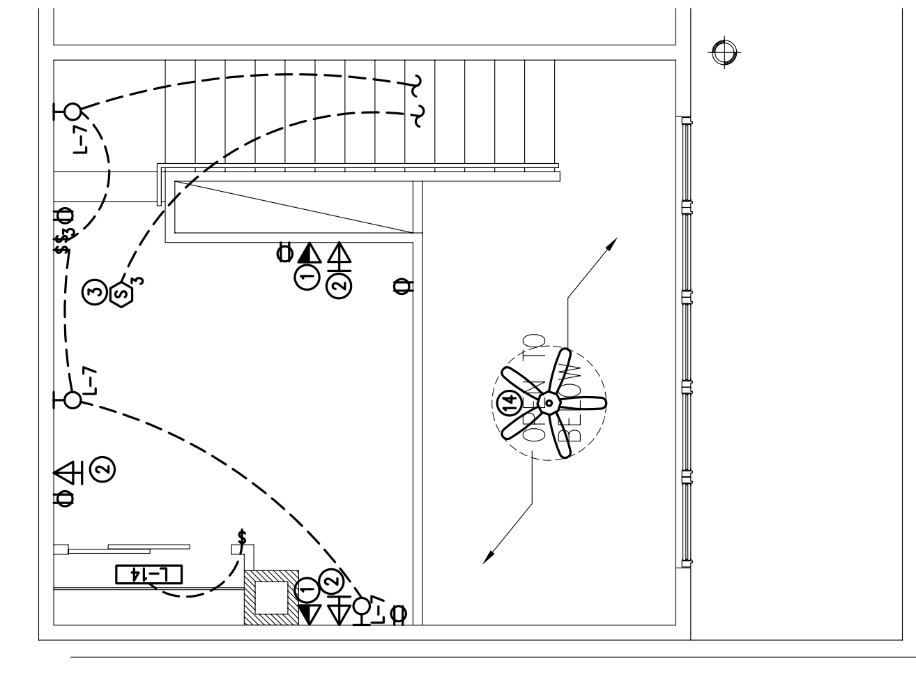
1 TYPICAL UNIT TYPE "I" - (UPPER FLOOR) ELECTRICAL PLAN SCALE: 1/4"=1'-0"
