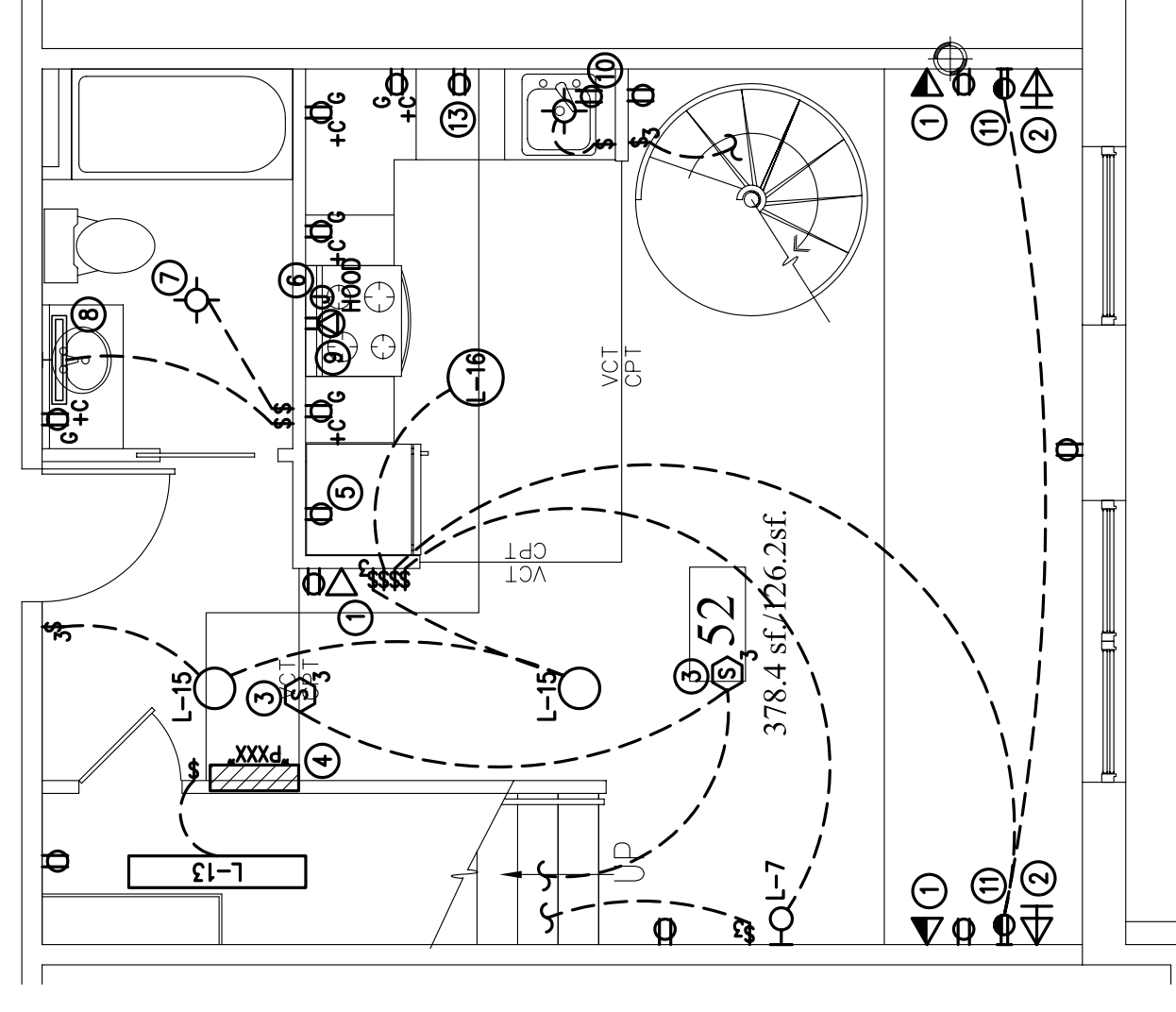
3 TYPICAL UNIT TYPE "K" - (LOWER FLOOR) ELECTRICAL PLAN SCALE: 1/4"=1'-0"
