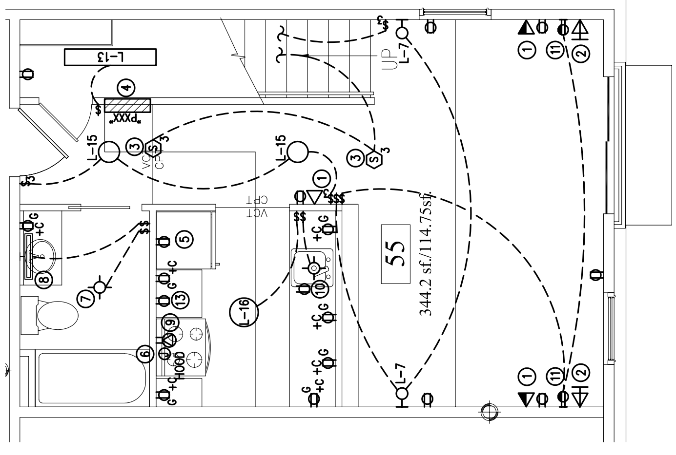
2 TYPICAL UNIT TYPE "J" - (LOWER FLOOR) ELECTRICAL PLAN SCALE: 1/4"=1'-0"
