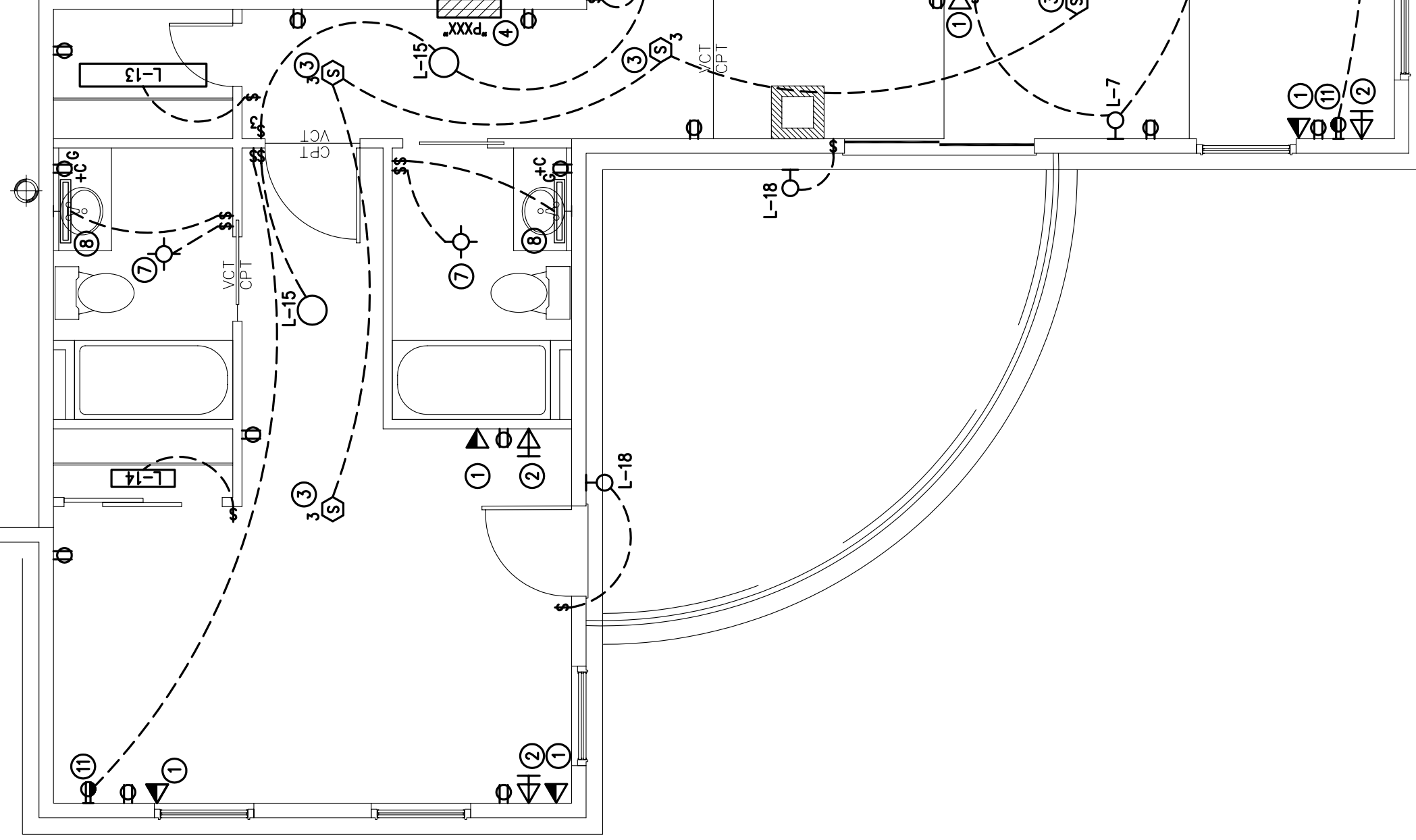
8 TYPICAL UNIT TYPE "H" - ELECTRICAL PLAN SCALE: 1/4"=1'-0"
