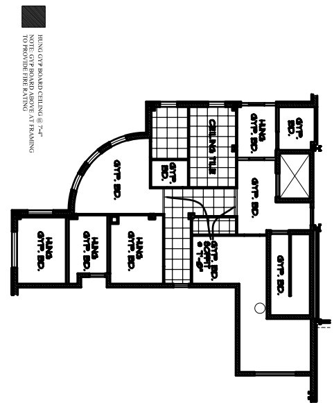
② GROUND FLOOR REFLECTED CEILING PLAN SCALE: 1/8" = 1'-0"
