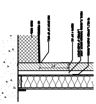
23 ROOF MASONRY WALL DETAIL SCALE: 1/8"=1'-0"
