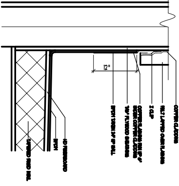
17 FLAT ROOF/COPPER CLAD WALL DETAIL SCALE: 3/4"=1'-0"
