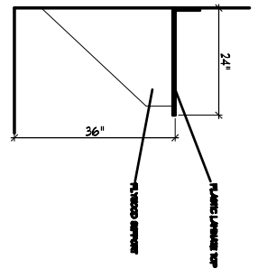
13 LAUNDRY COUNTER SECTION SCALE: 1/4"=1'-0"
