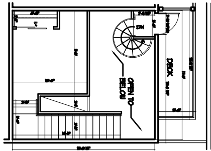
④ UNIT TYPE M (UPPER FL.) SCALE: 1/8" = 1'-0"
