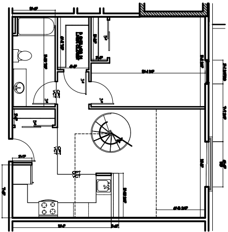
⑤ UNIT TYPE N (LOWER FL.) SCALE: 1/8" = 1'-0"
