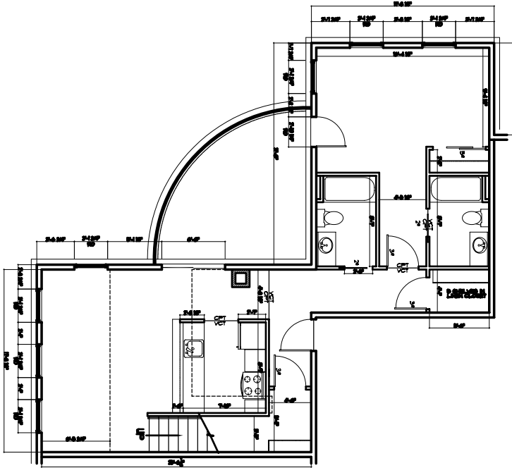
① UNIT TYPE J (LOWER FL.) SCALE: 1/4" = 1'-0"
