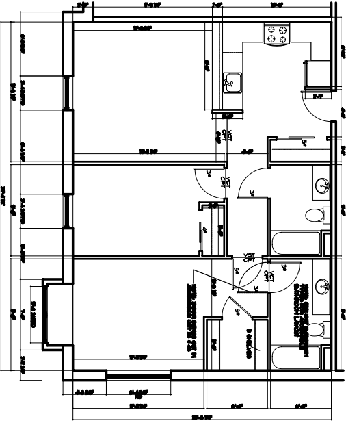
③ UNIT TYPE C SCALE: 1/4" = 1'-0"
