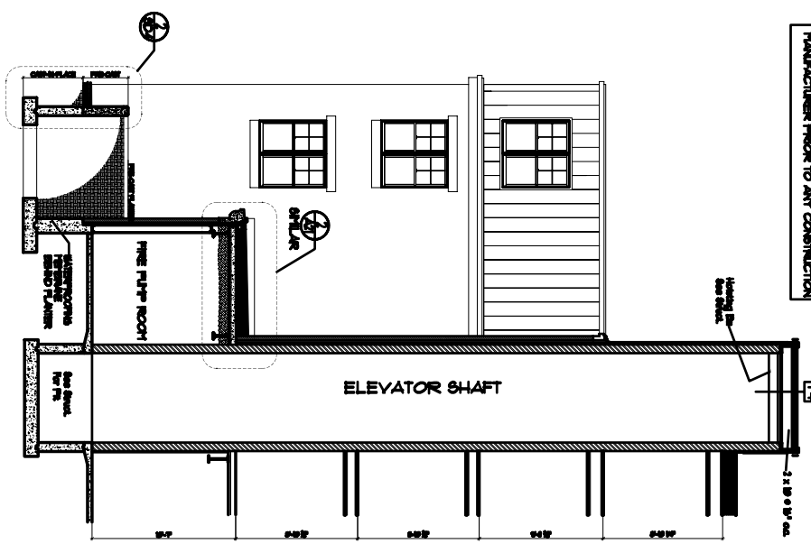
⑤ ELEVATOR SHAFT SECTION SCALE 1/4"=1'-0"
