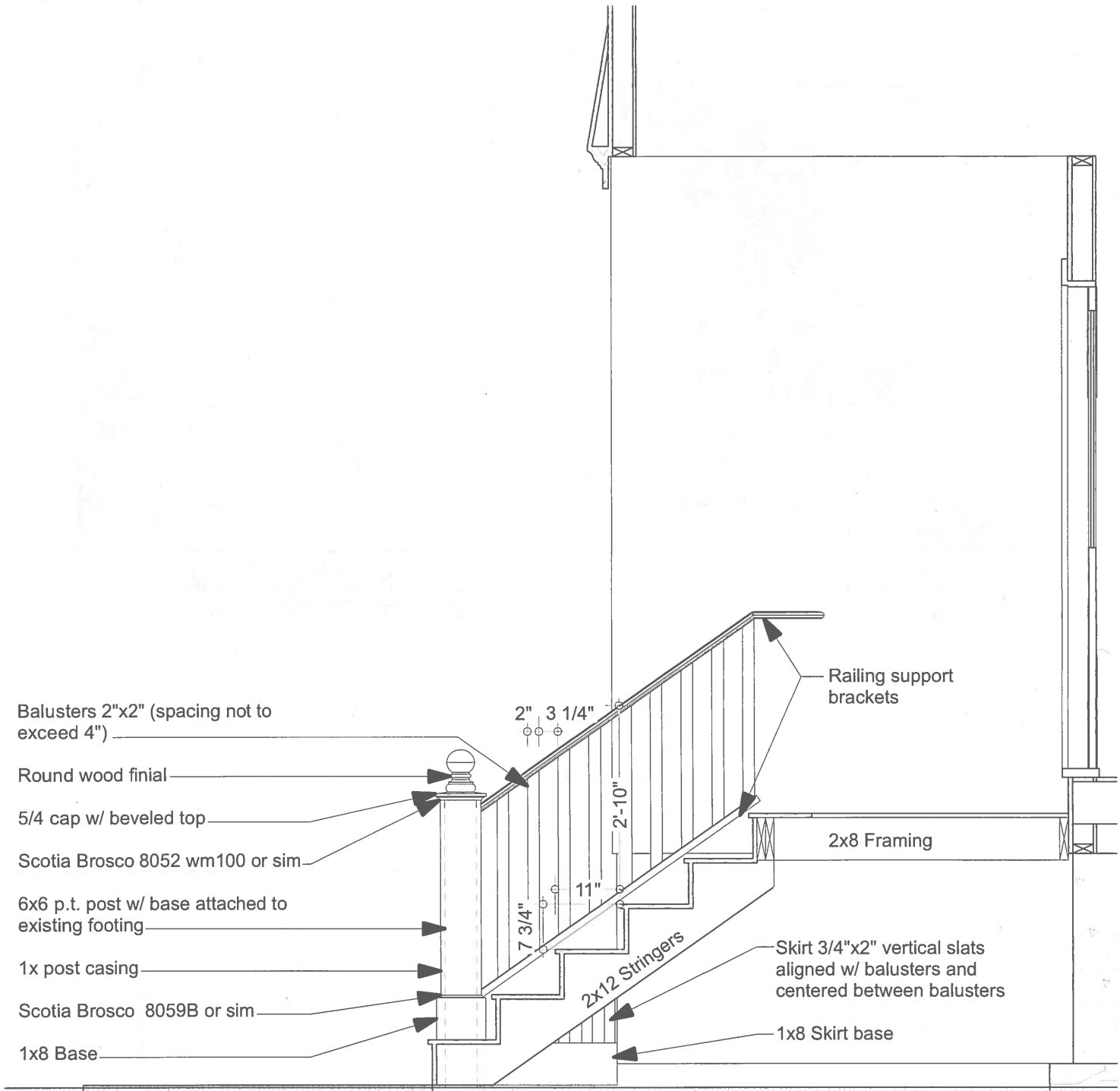
1 Front Stair Section SCALE: 1/2" = 1'-0"
