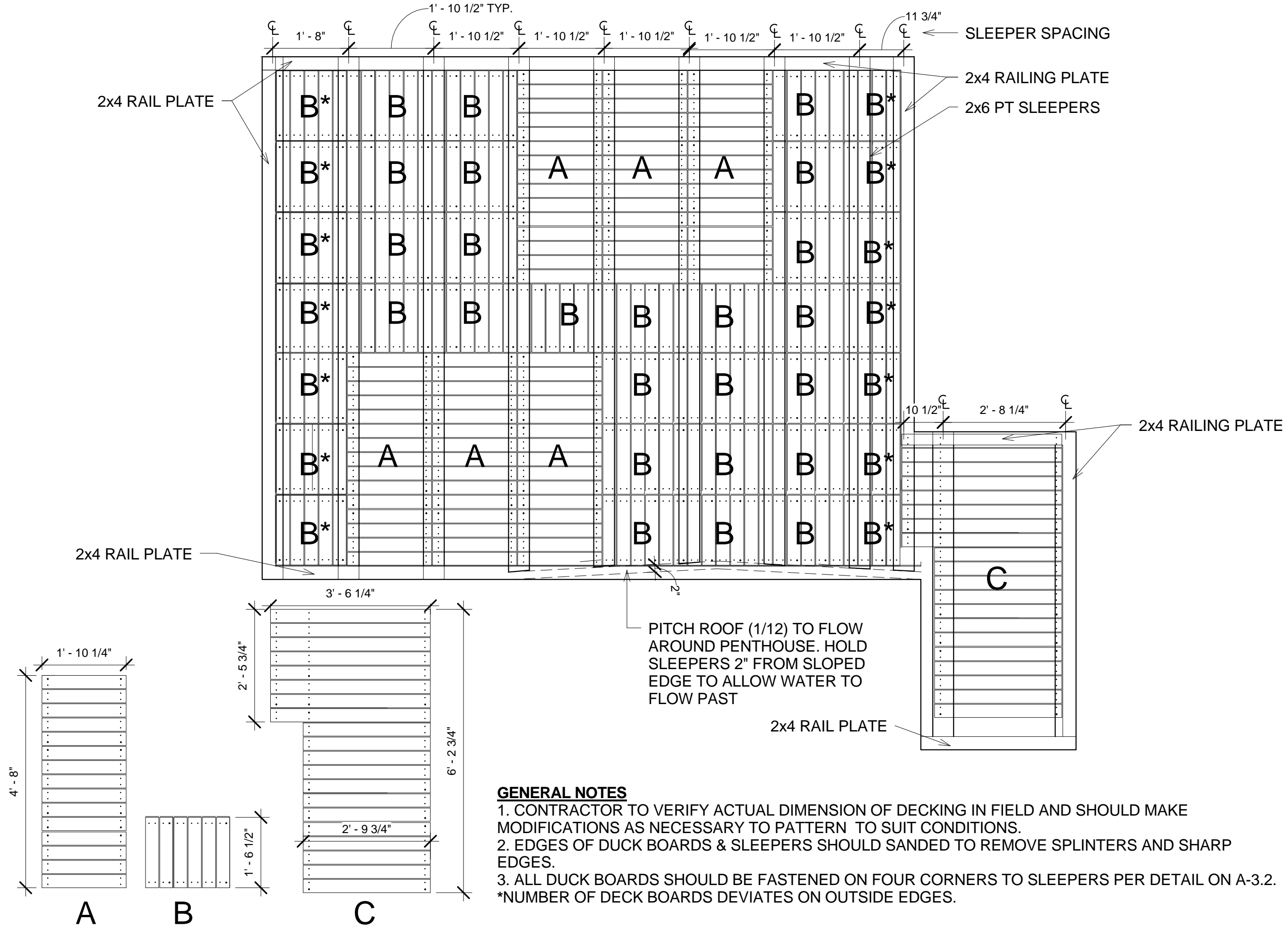
1 DECKING PATTERN & SLEEPER LAYOUT 1/2" = 1'-0"
