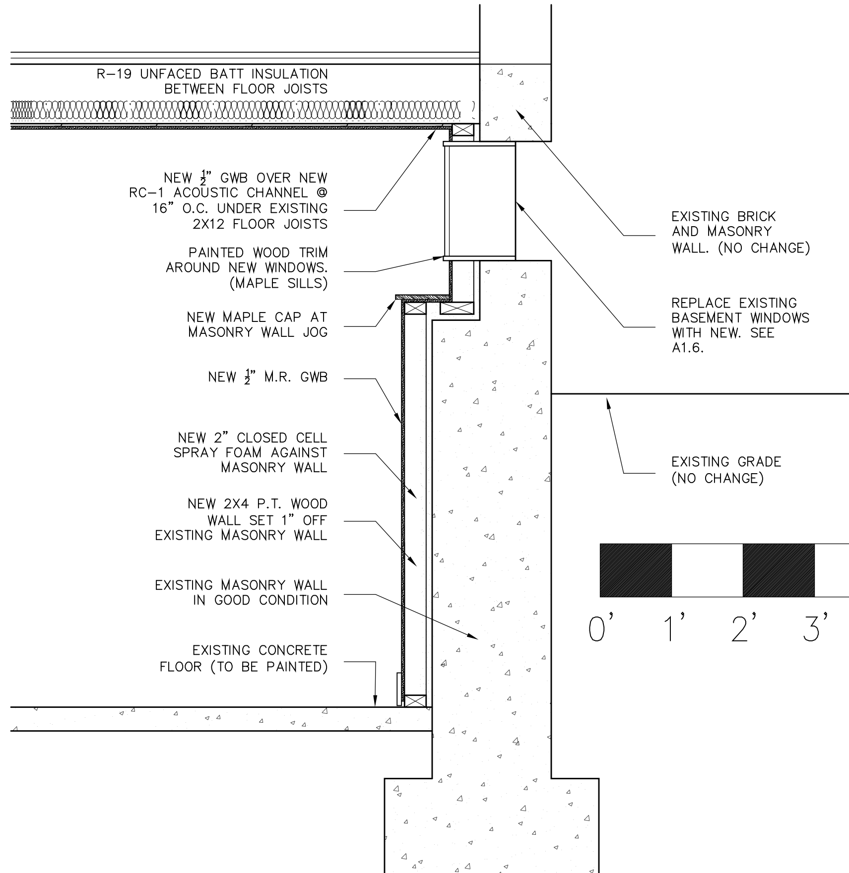
1 EXTERIOR WALL SECTION SCALE: 3/4" = 1' - 0"
