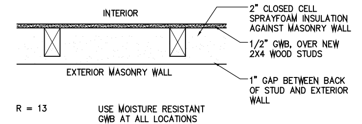
2 TYPICAL EXTERIOR WALL ASSEMBLY
