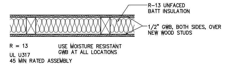
3 TYP. INTERIOR WALL
