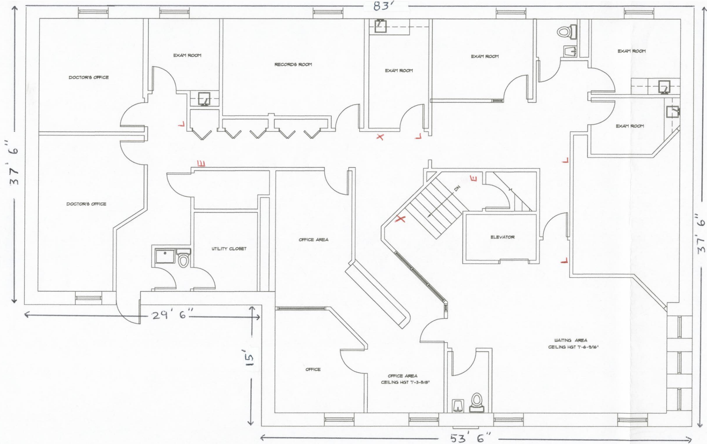
19 West St. Basement Level 1/8" = 1'-0"
