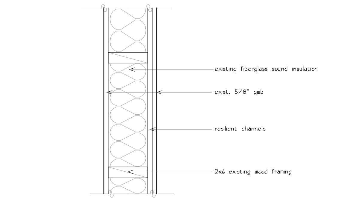
5 existing unit division partition 1 hr rated
