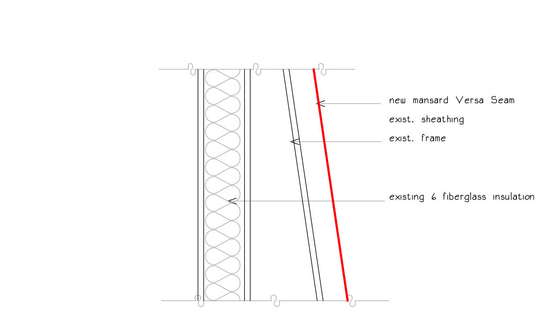
8 3rd floor mansard section
