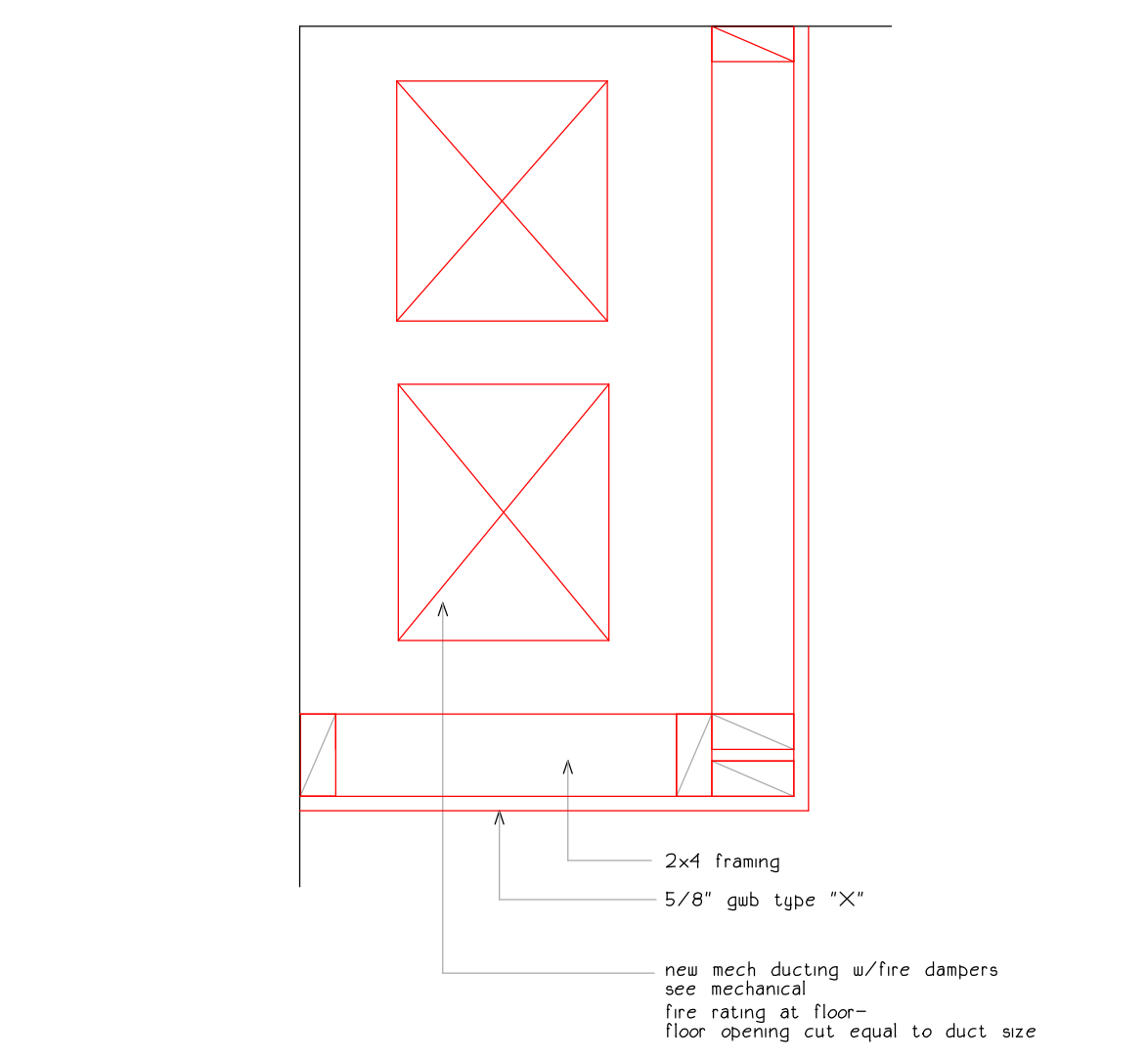
16 new duct enclosure plan view, see mechanical
