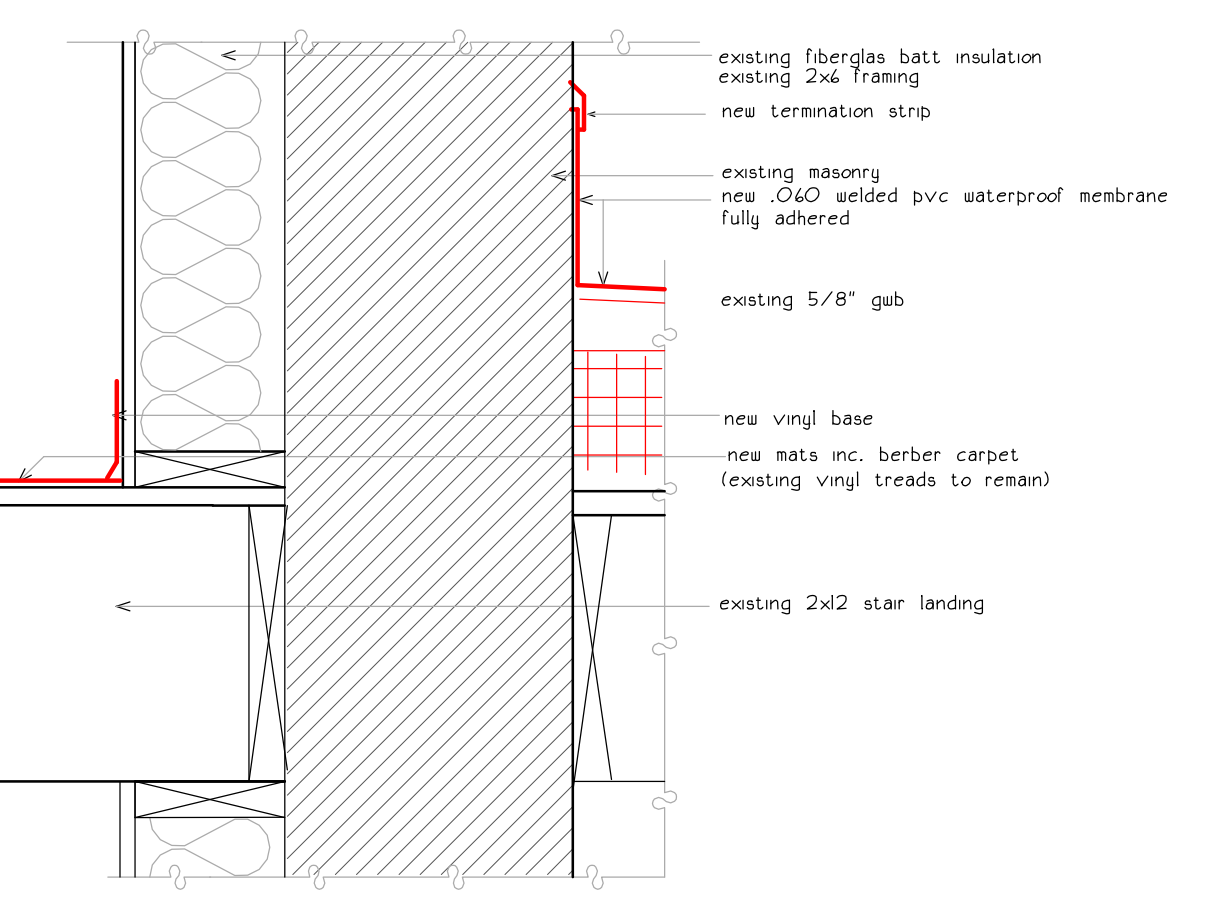
11 stair at 4th floor exterior (presumed 2hr)
