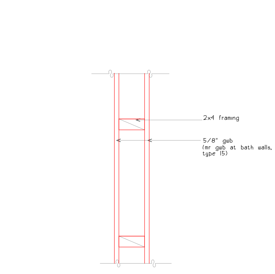
14 new wall at units plan 15 new wall baths (mr gw) b
