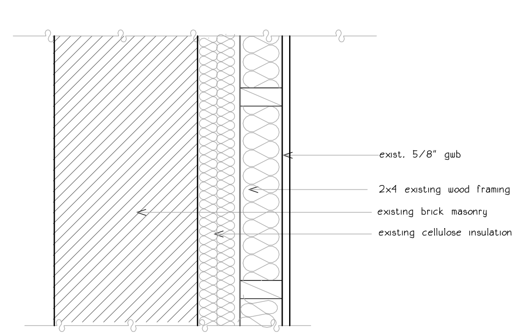
1 existing exterior wall
