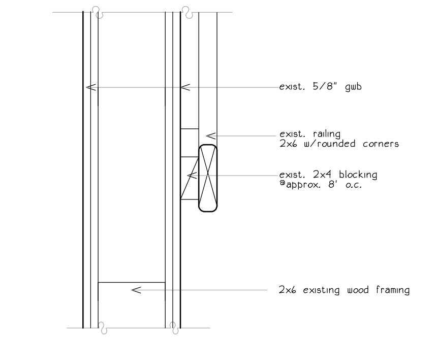
4 existing stair wall/handrail section 2 hr rated
