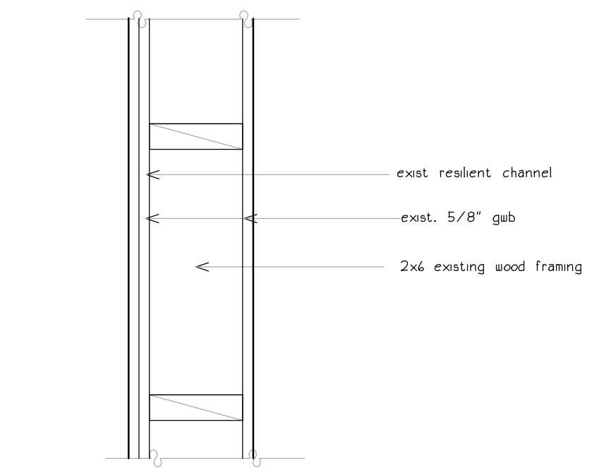
2 existing corridor wall 1 hr rated
