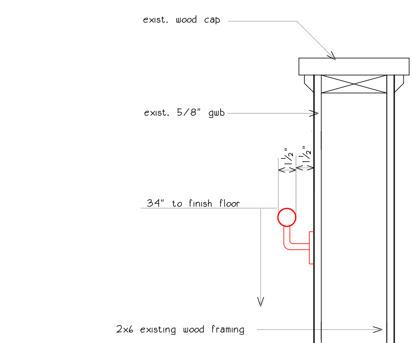
9 railing at ramp section
