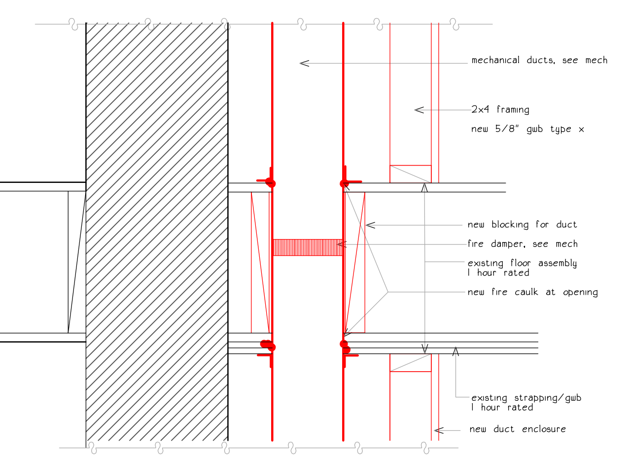
16a new duct enclosure, 1hr rating at floor section view, see mechanical
