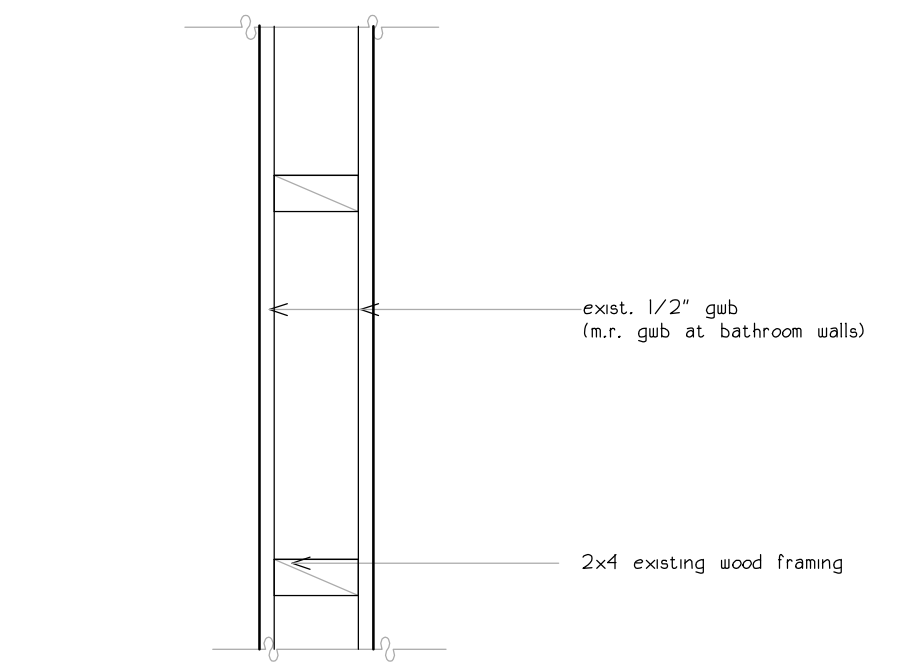
3 existing interior unit wall
