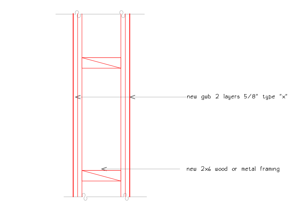
6 new stair wall 2 hr rated
