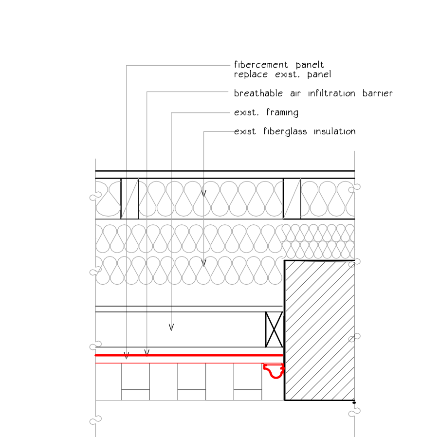
13 fiber cement panels below windows plan at jamb exist masonry jamb
