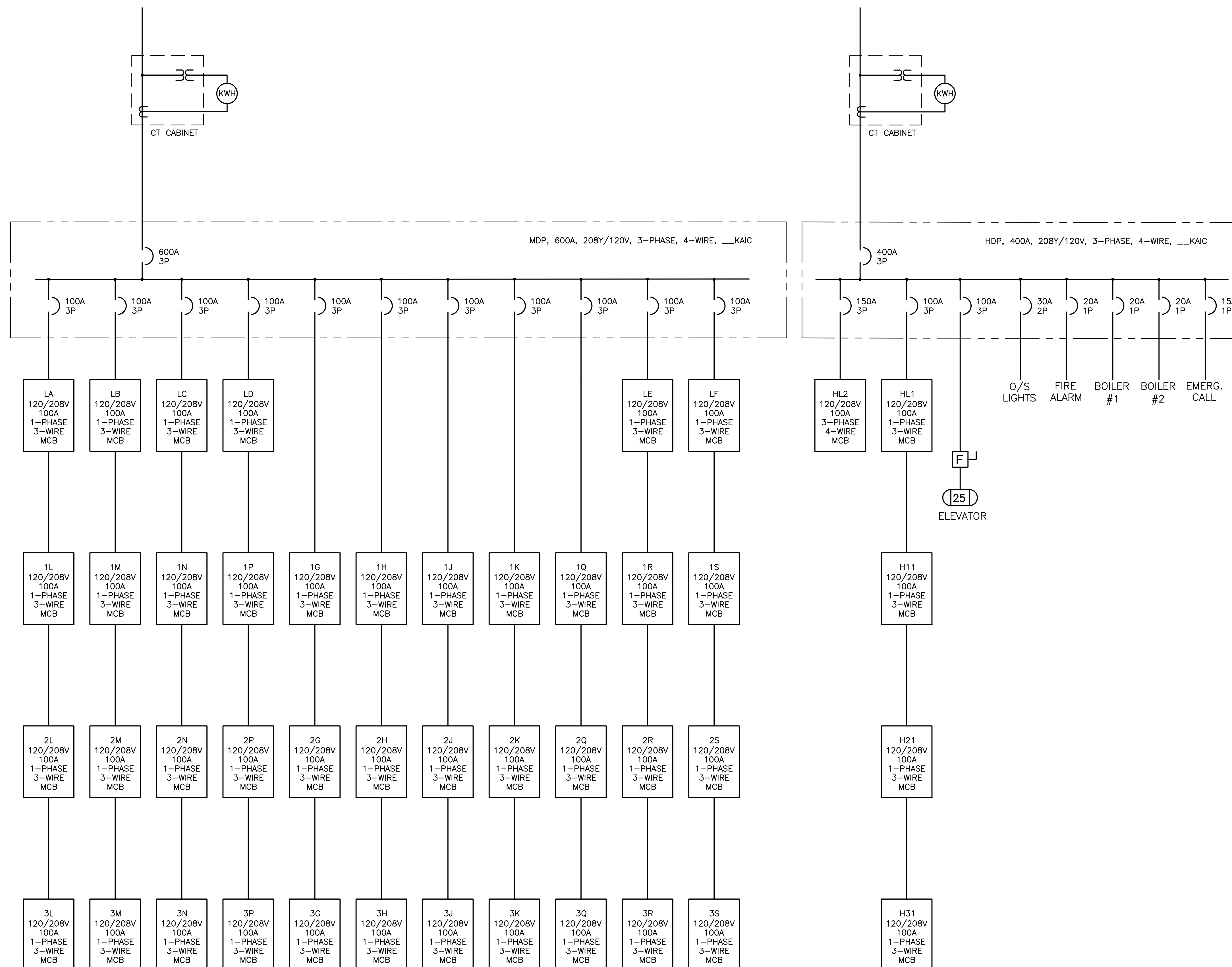
1 EXISTING ELECTRICAL ONE-LINE DIAGRAM SCALE: NOT TO SCALE
