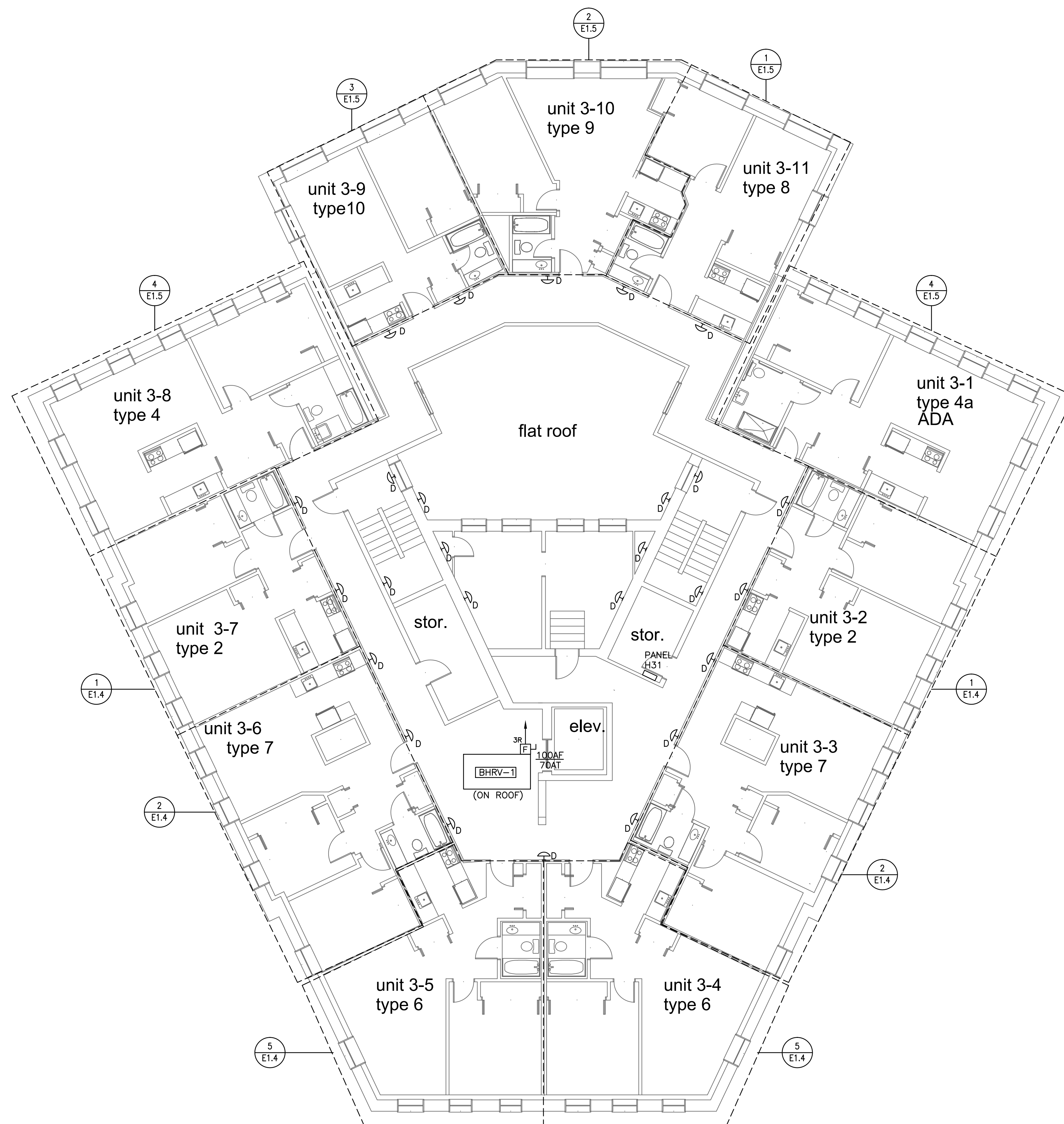
1 ELECTRICAL POWER & SYSTEMS PLAN - THIRD FLOOR SCALE: 1/8"=1'
