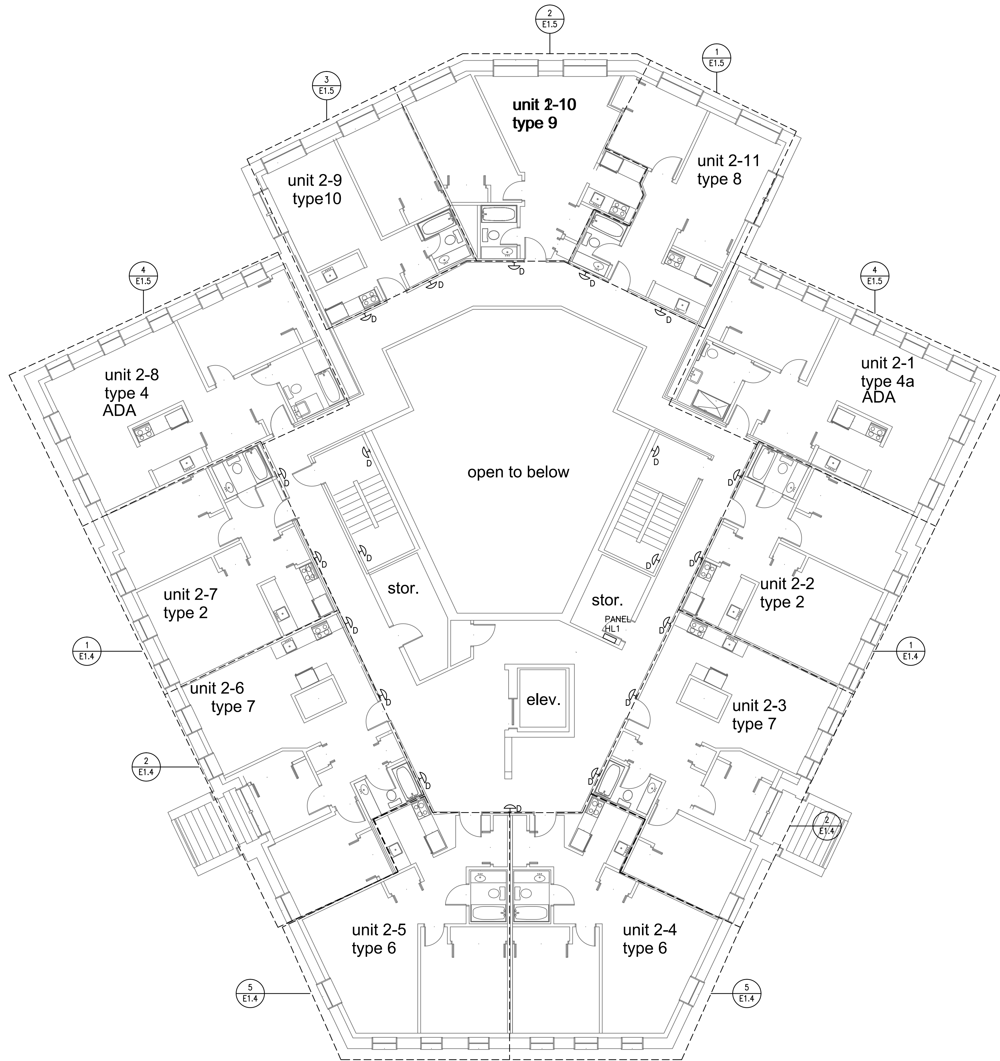
1 ELECTRICAL POWER & SYSTEMS PLAN – SECOND FLOOR SCALE: 1/8"=1'
