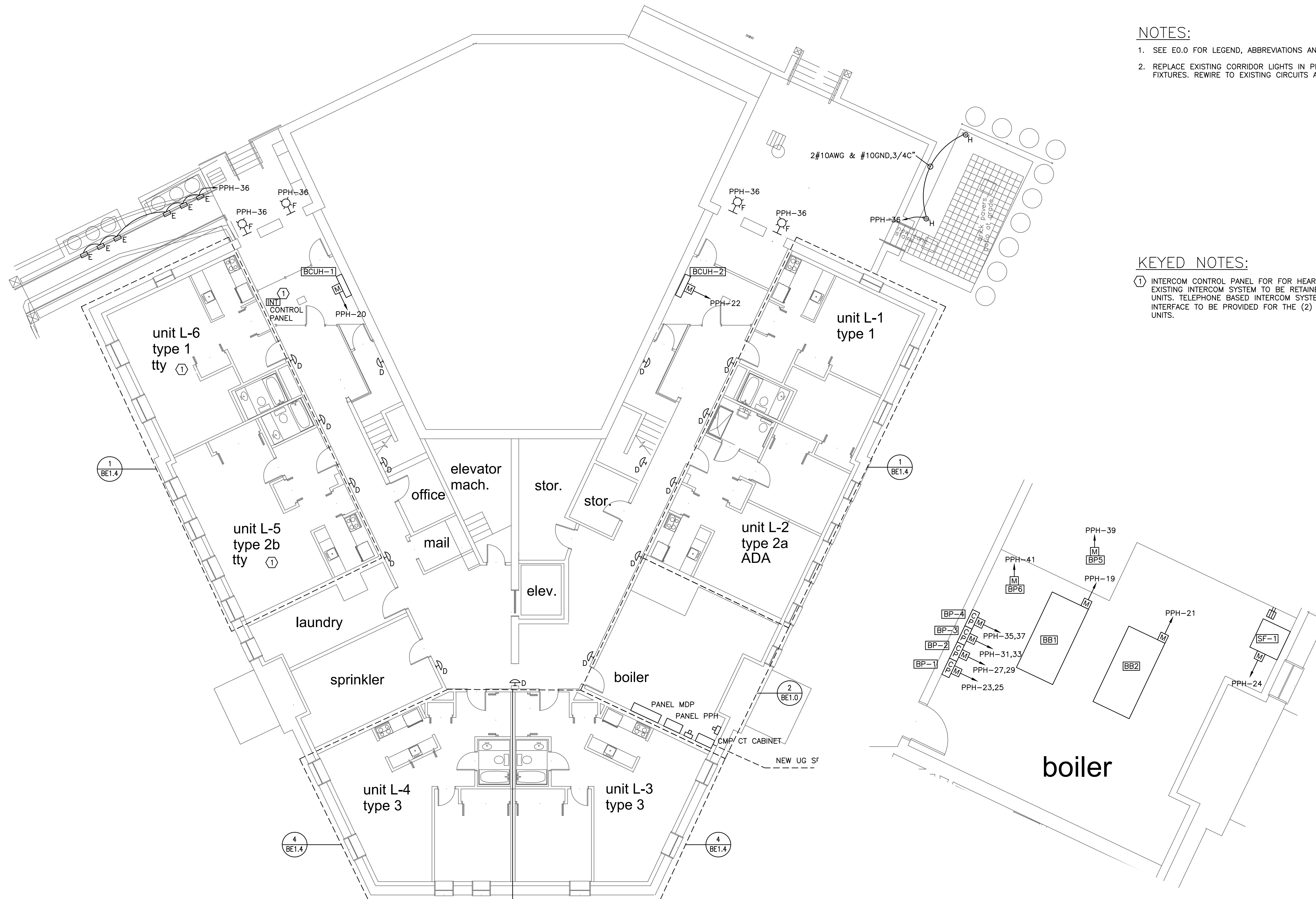
1 ELECTRICAL DETAIL - BOILER ROOM SCALE: 1/4"=1'
