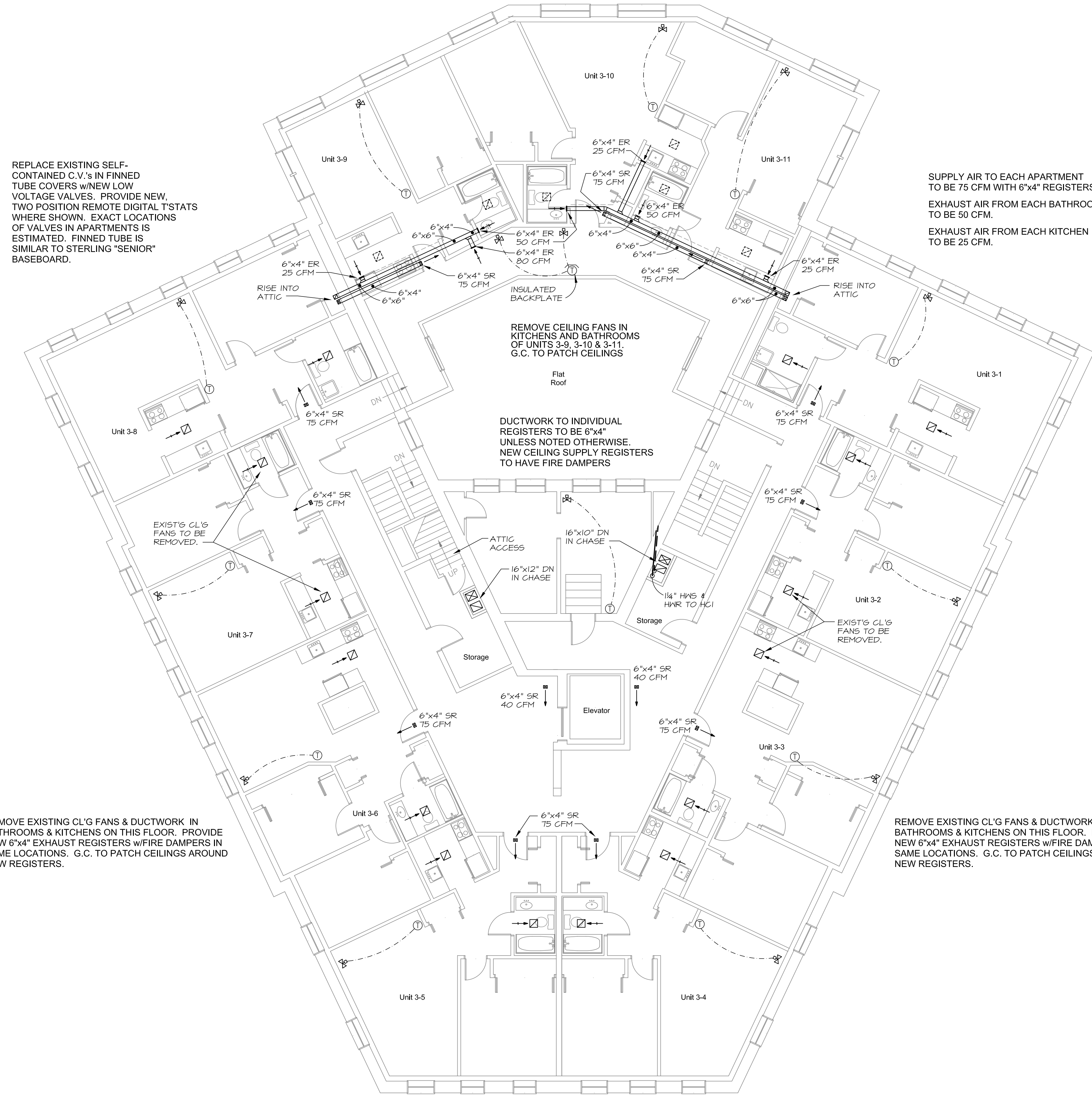
3 LEVEL 3 MECHANICAL PLAN SCALE: 1/8" = 1'-0"
