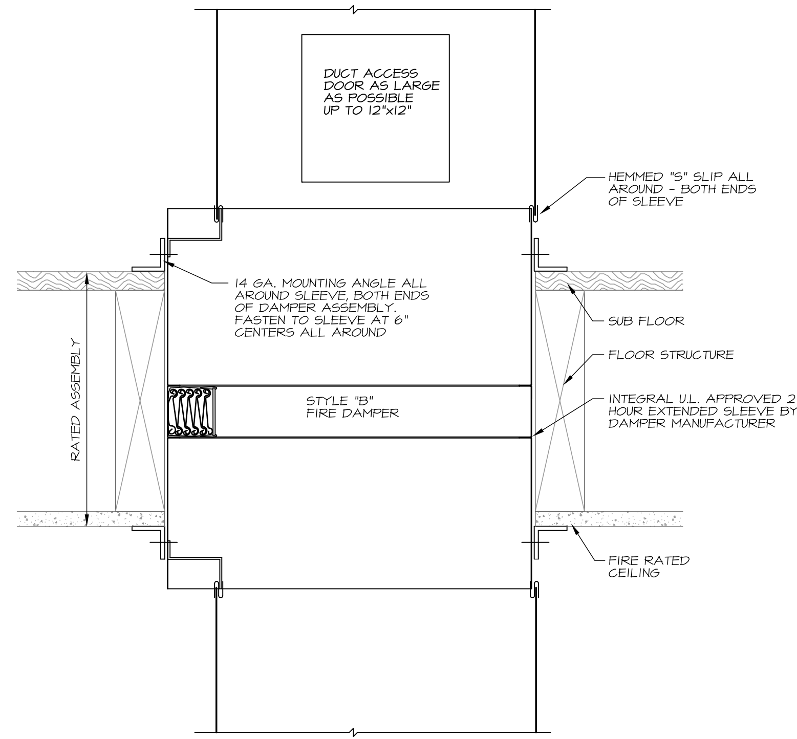
1 FLOOR FIRE DAMPER STYLE "B" NO SCALE
