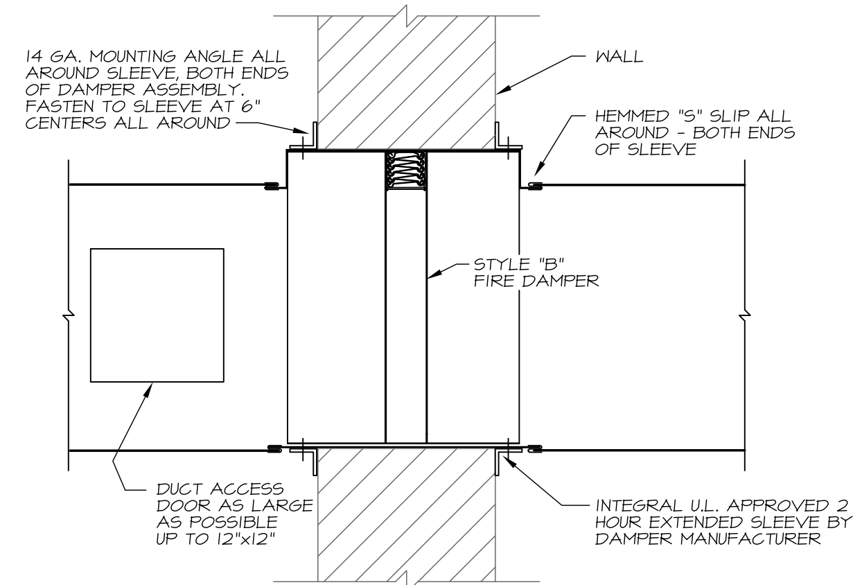
2 WALL FIRE DAMPER STYLE "B" NO SCALE
