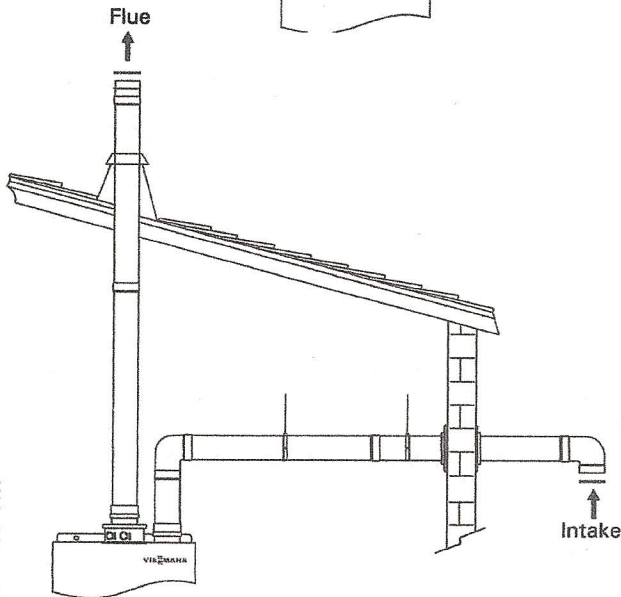
Two pipe system (room air independent) hybrid
