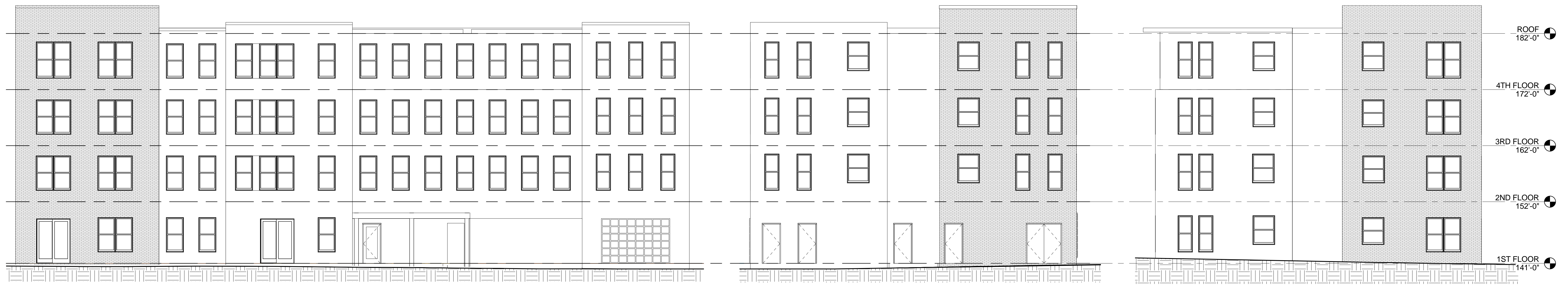
2 | EAST ELEVATION 1/8" = 1'-0" 0 2' 4' 8' 16'
