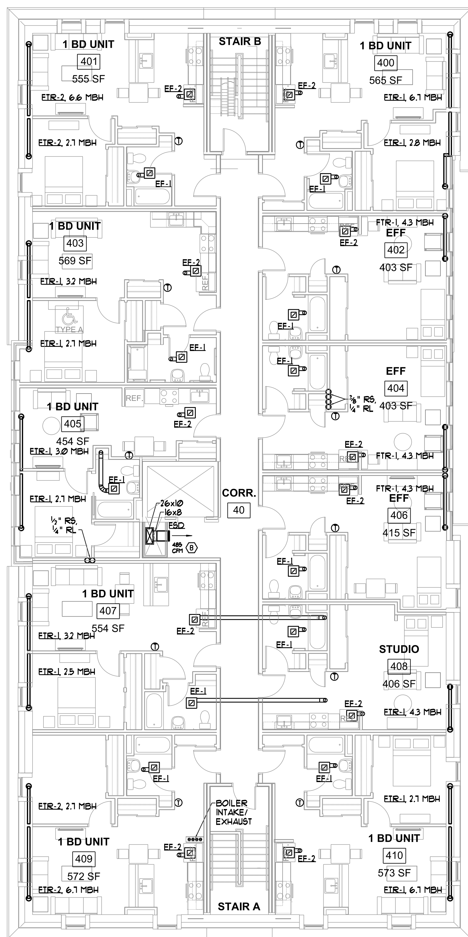
FOURTH FLOOR MECHANICAL PLAN SCALE - 1/8" = 1'-0"
