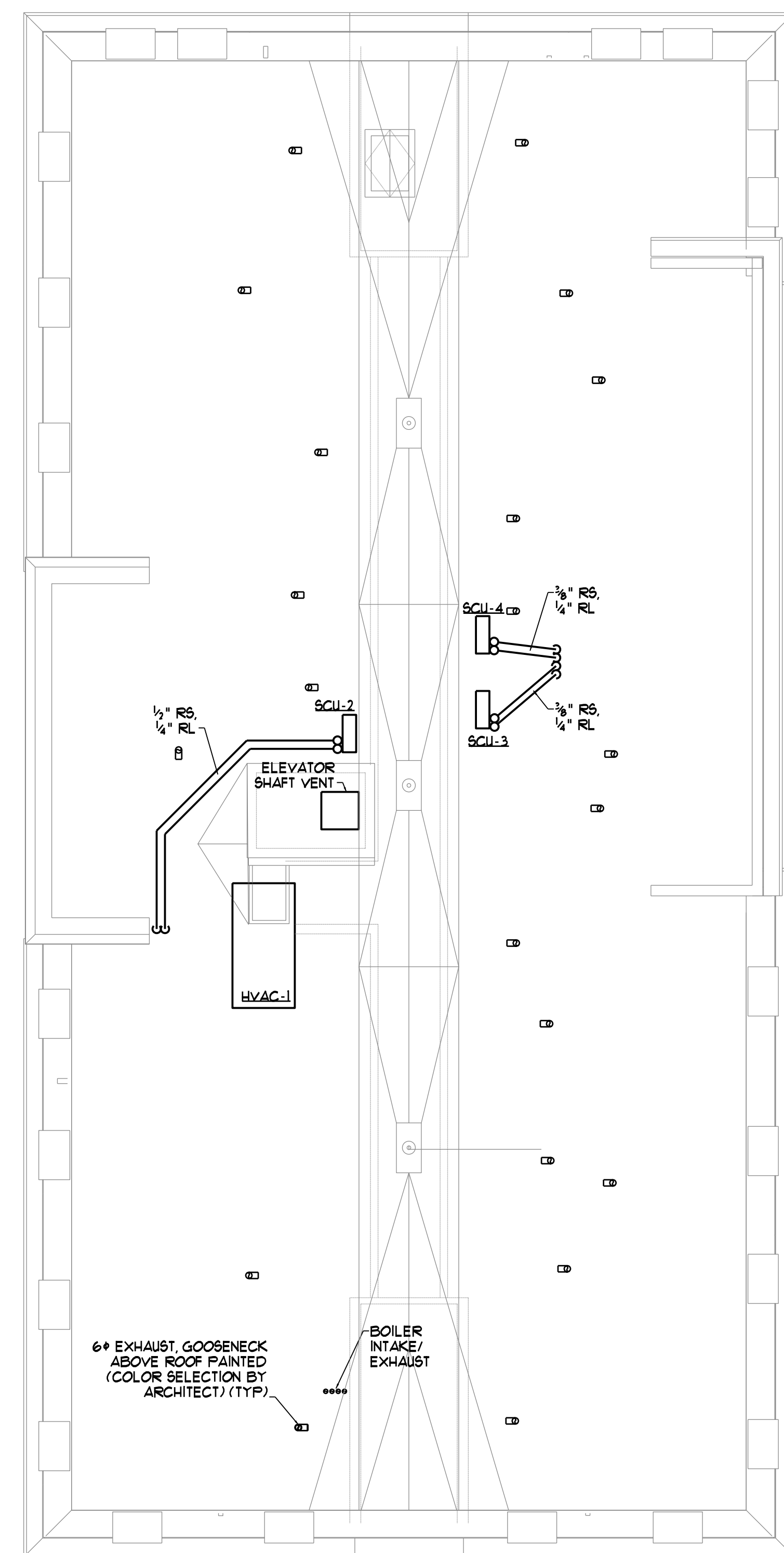
ROOF MECHANICAL PLAN SCALE - 1/8" = 1'-0"
