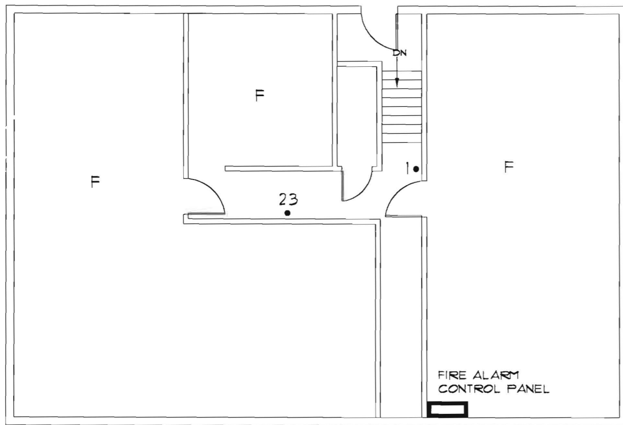
BASEMENT PLAN
