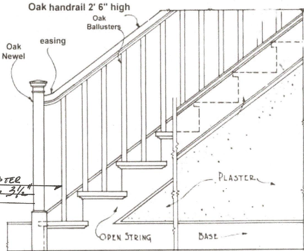
Detail view of stairs
