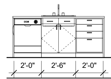
4 | SECOND/THIRD FLOOR KITCHEN ELEVATION B 1/4" = 1'-0"
