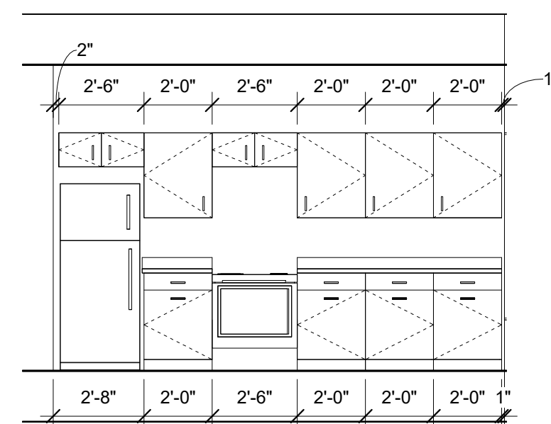
3 | SECOND/THIRD FLOOR KITCHEN ELEVATION A 1/4" = 1'-0"
