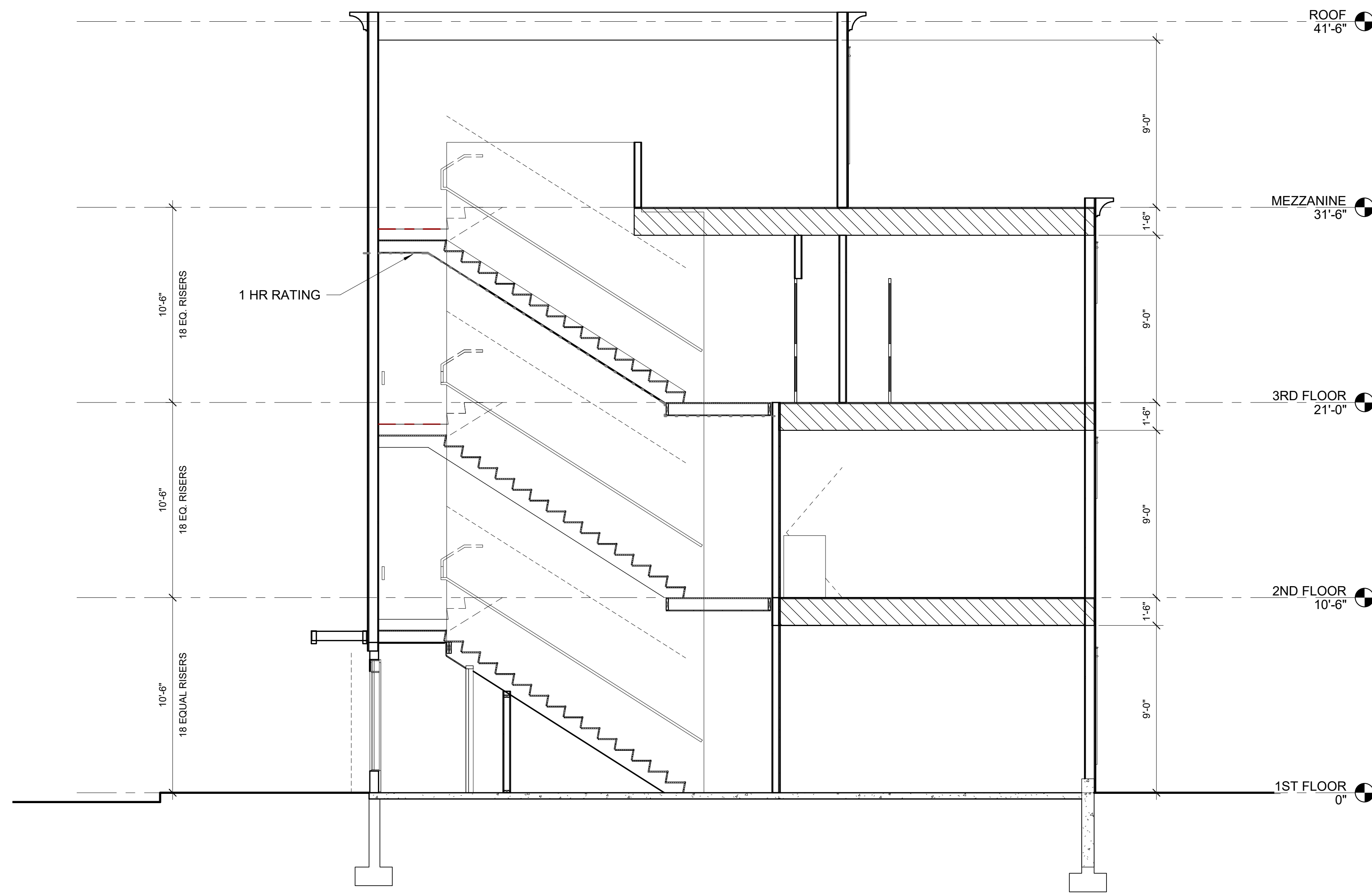
1 | Section 1 1/4" = 1'-0"
