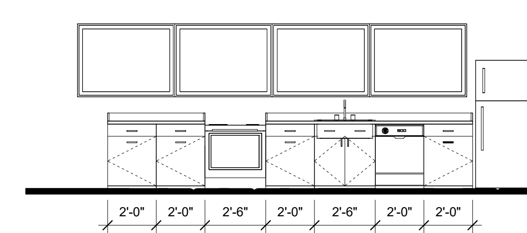
2 | FIRST FLOOR KITCHEN 1/4" = 1'-0"
