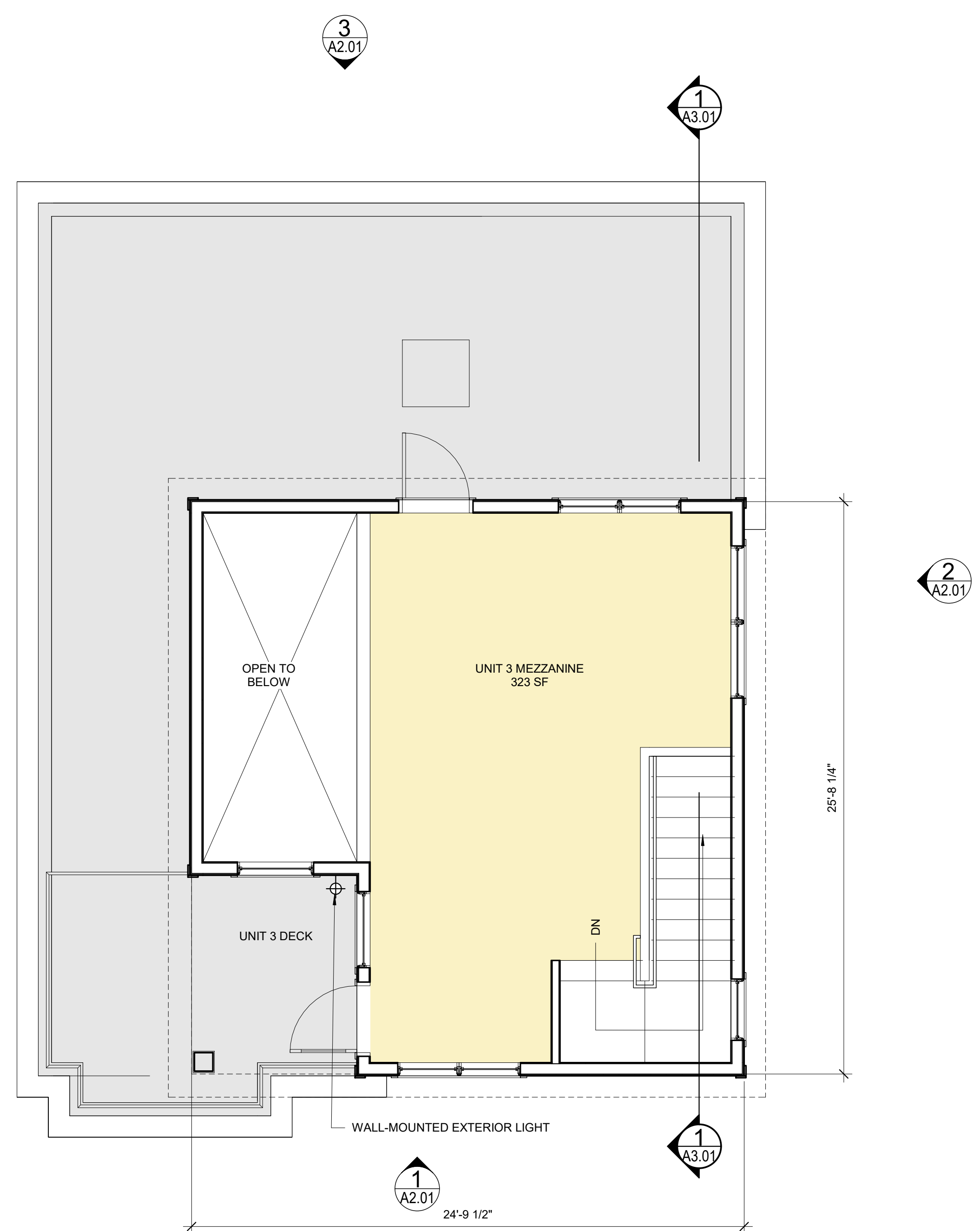
2 | MEZZANINE 1/4" = 1'-0"
