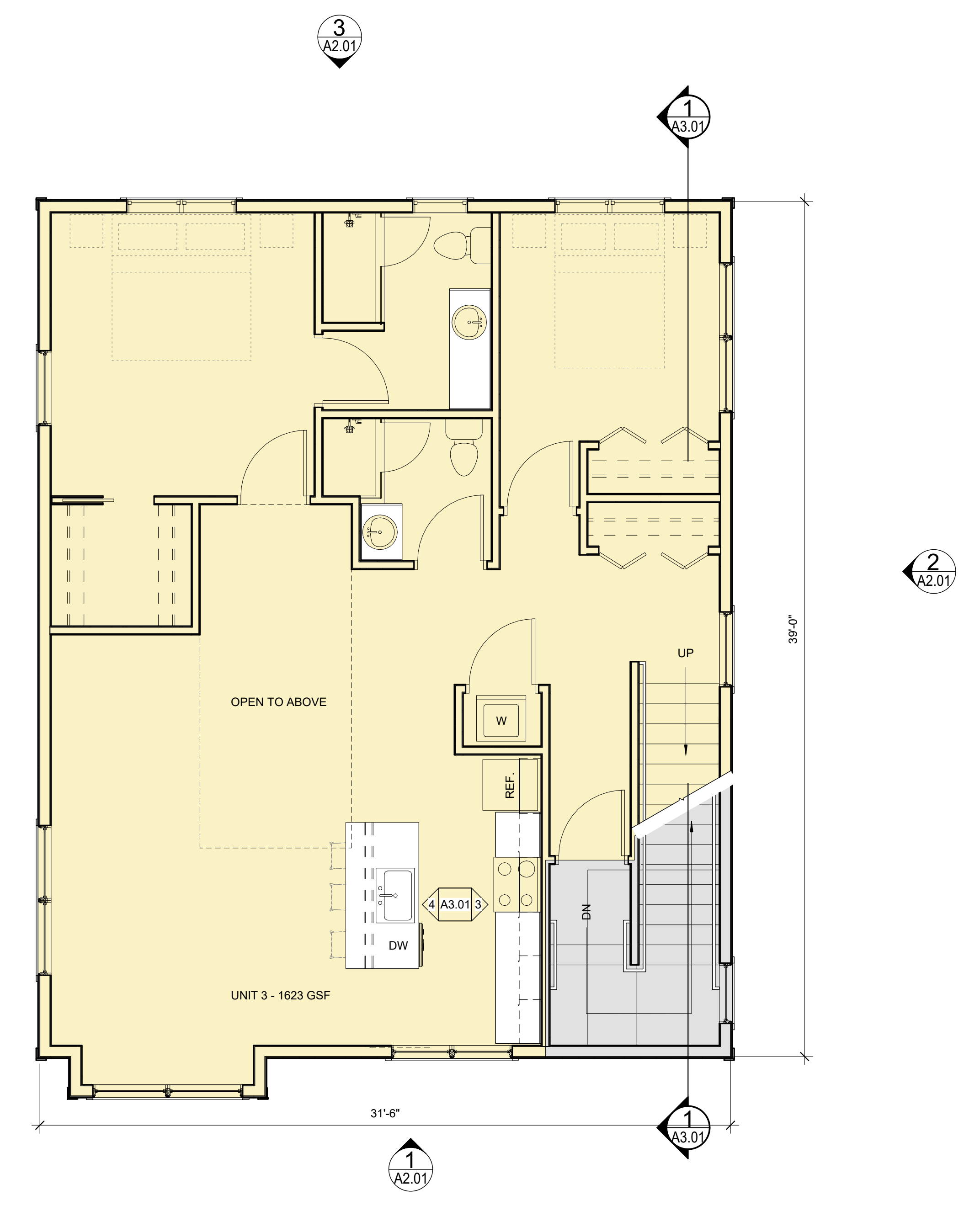
1 | 3RD FLOOR 1/4" = 1'-0"
