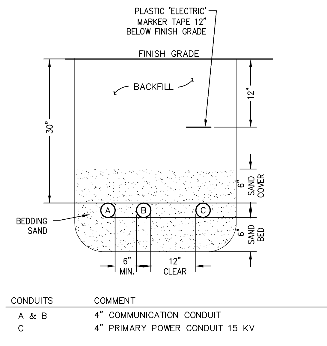
DUCT BANK SECTION C4 NOT TO SCALE
