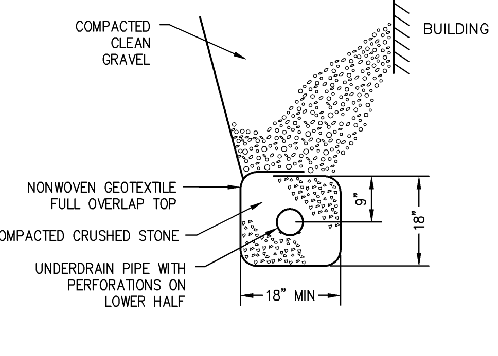
UNDERDRAIN OR FOUNDATION DRAIN D2 NOT TO SCALE
