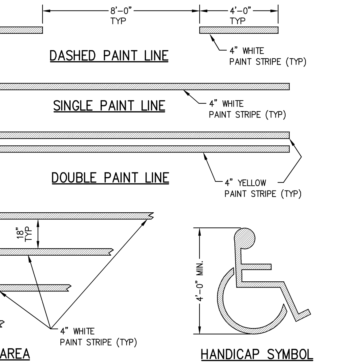
STANDARD PAINT STRIPING B1 NOT TO SCALE
