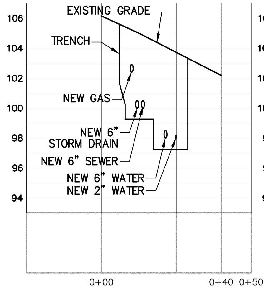
NEW UTILITY SECTION D3 SCALE: H: 1"=20'/V: 1"=4'
