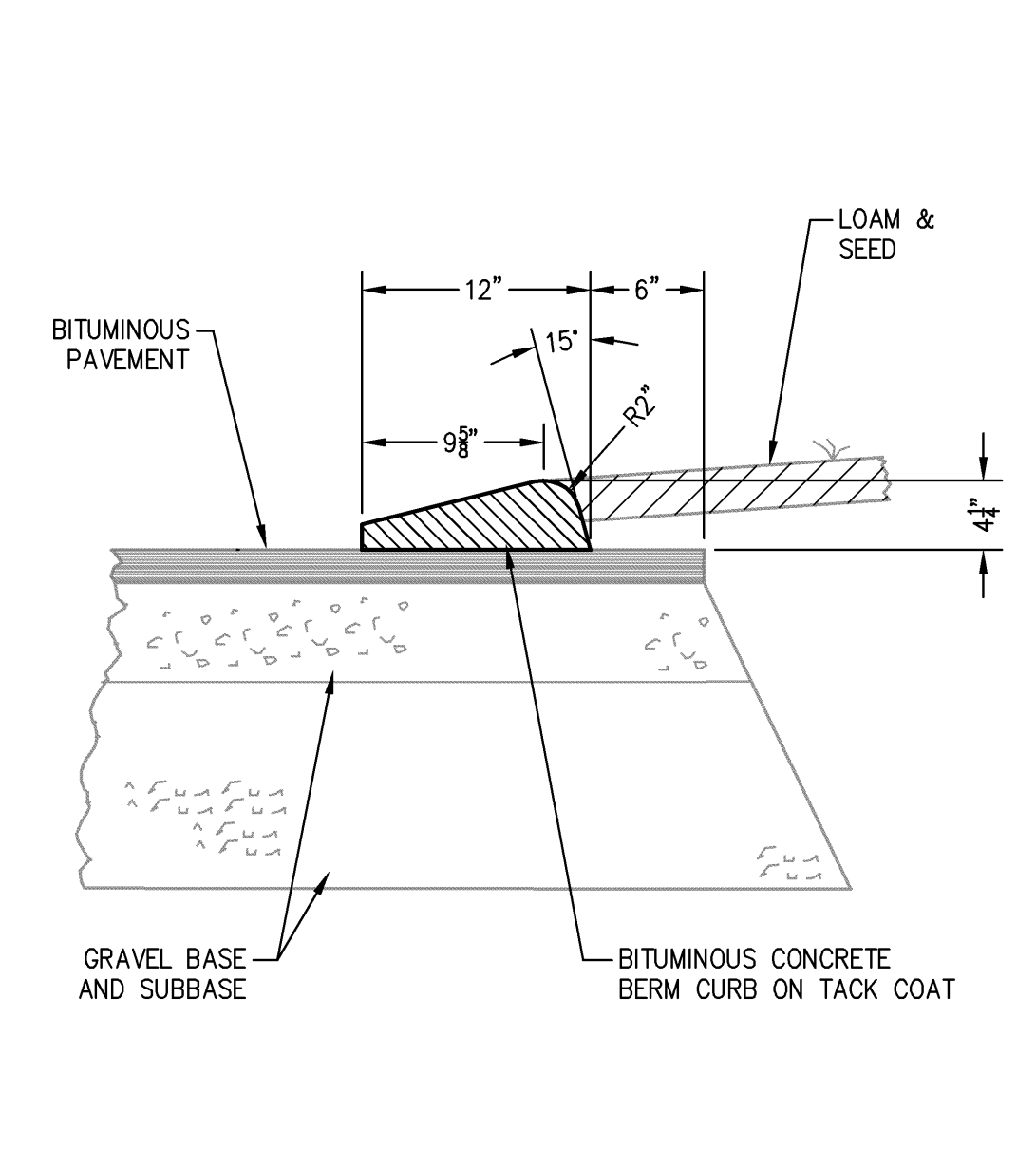
C.I.P. CONCRETE SURFACING A6 NOT TO SCALE
