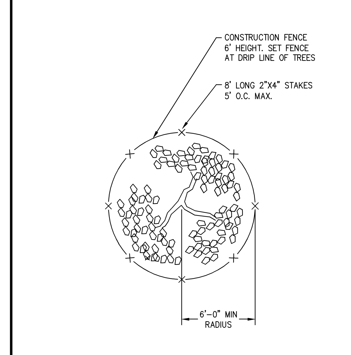
TEMPORARY TREE PROTECTION DETAIL B5 NOT TO SCALE
