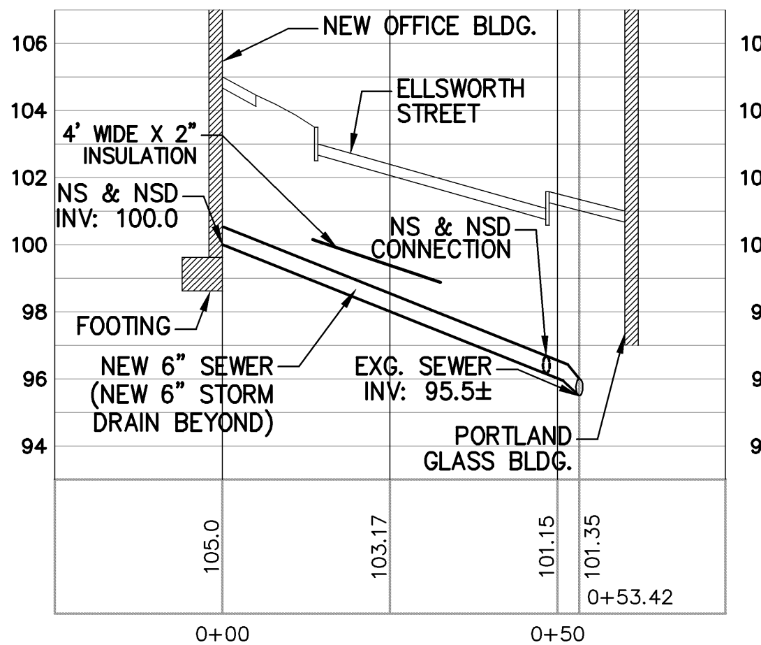
NEW SEWER & NEW STORM DRAIN PROFILE D5 SCALE: H: 1"=20'/V: 1"=4'
