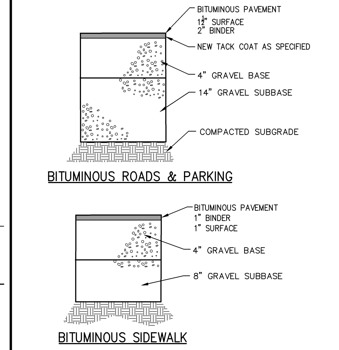
BITUMINOUS PAVEMENT DETAILS A5 NOT TO SCALE
