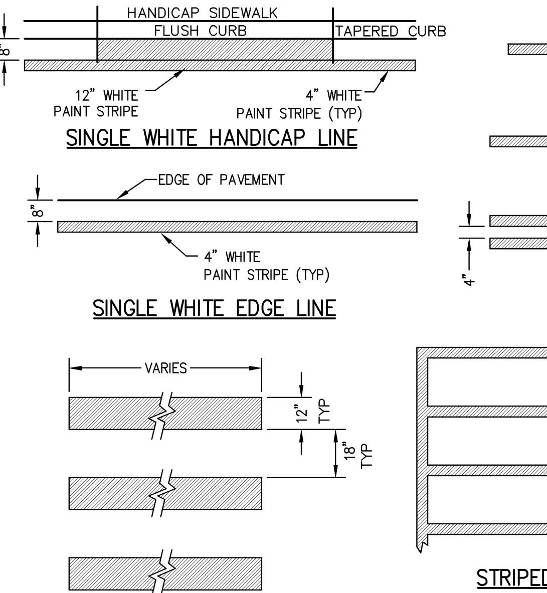
PEDESTRIAN CROSSWALK B1 NOT TO SCALE
