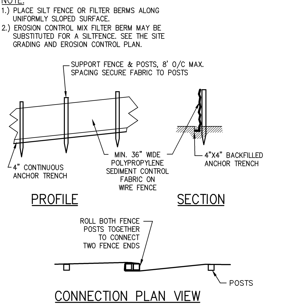
SILT FENCE B4 NOT TO SCALE
