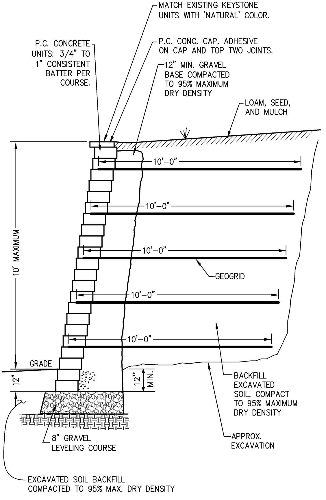
PRECAST CONCRETE UNIT RETAINING WALL C1 NOT TO SCALE
