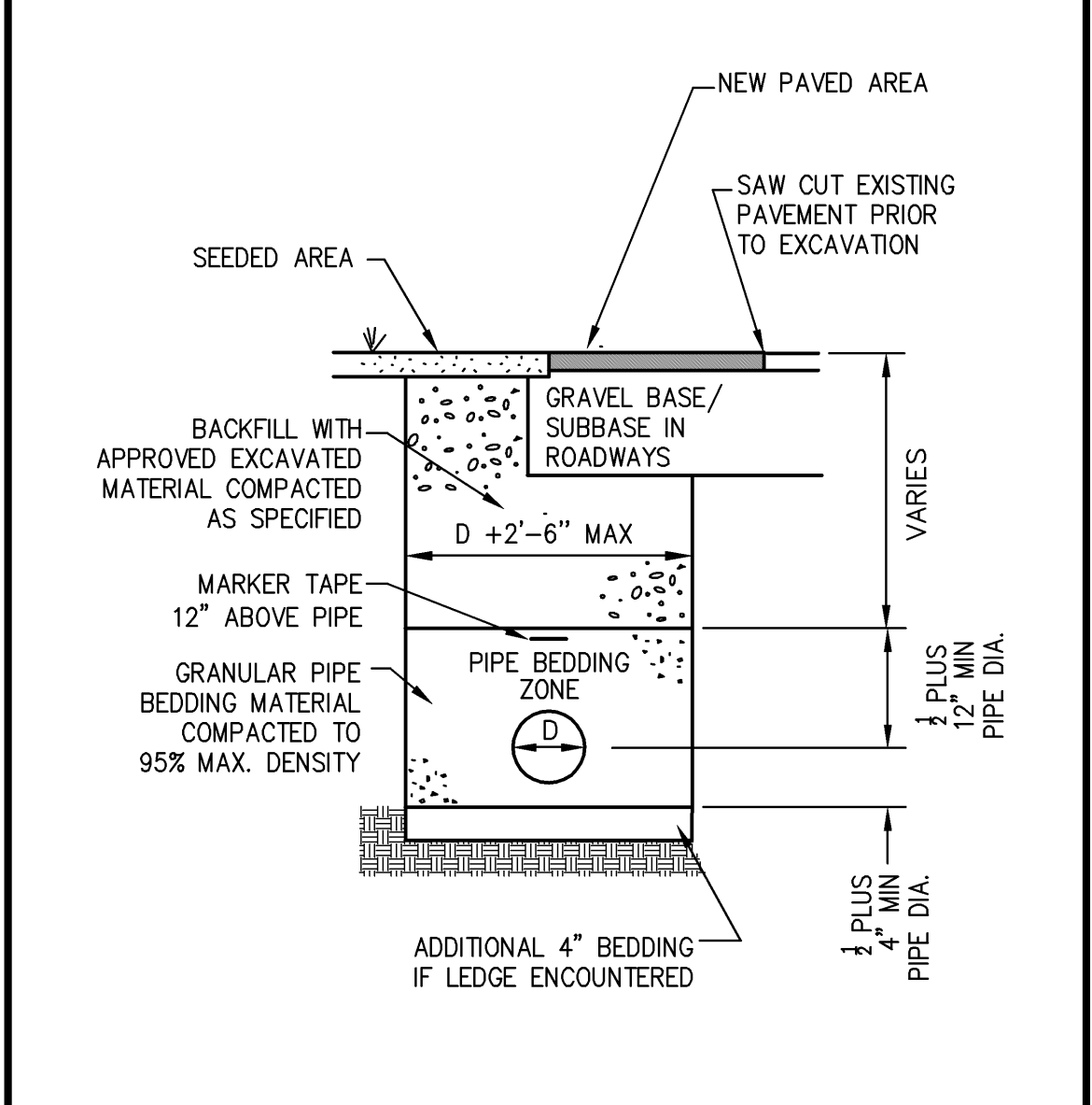
PIPE TRENCH B3 NOT TO SCALE
