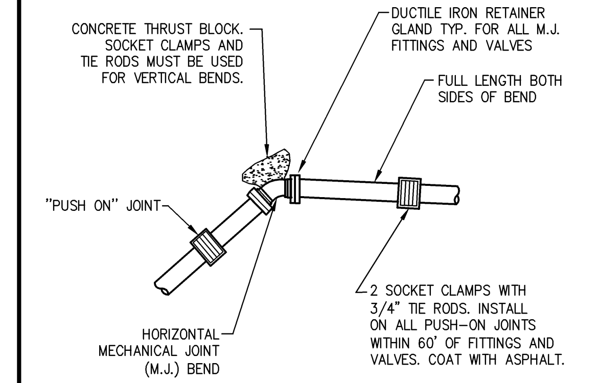
RESTRAINT AT FITTINGS WATER LINES C5 NOT TO SCALE
