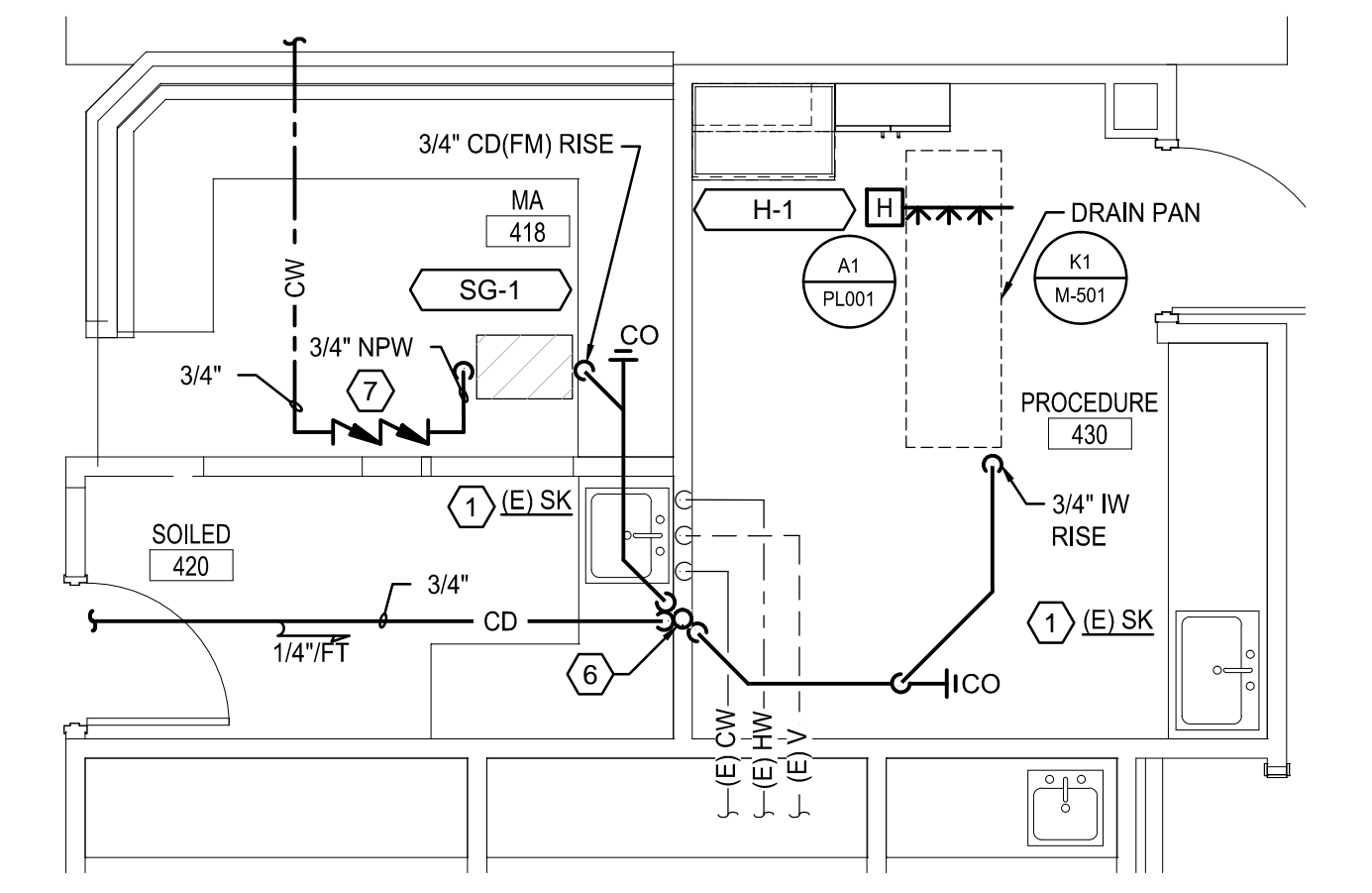
LEVEL 4 - PLUMBING PART PLAN (A10) 1/4" = 1'-0"
