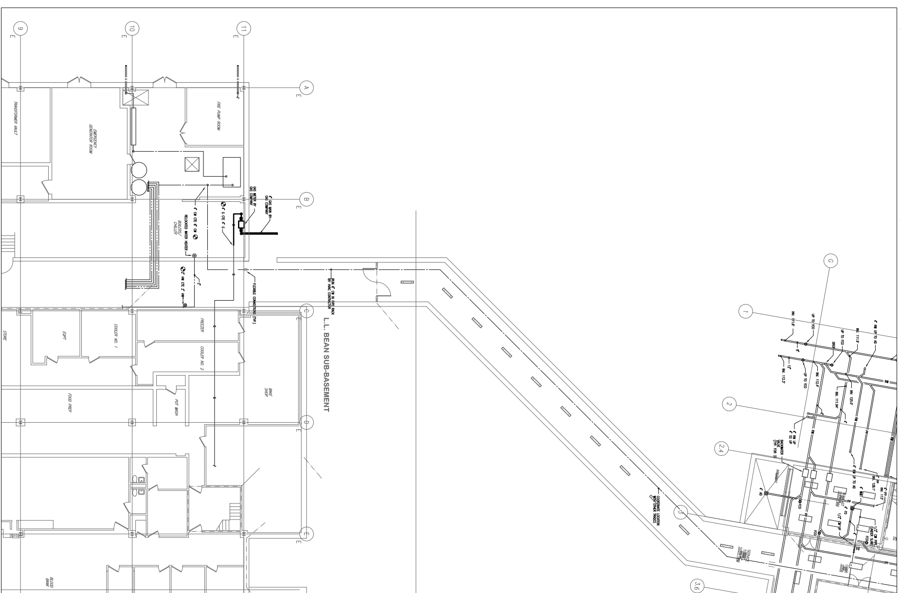
PLUMBING SUB-BASEMENT - RENOVATION
