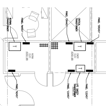
2 NORMAL AND EMERGENCY ELECTRICAL CLOSETS (SOUTH) SCALE: 1/4" = 1'-0"
