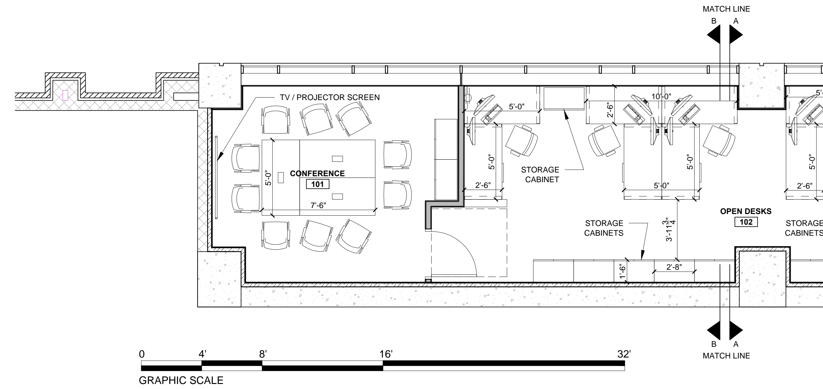
2 FIRST FLOOR FURNITURE PLAN - PART B 1/4" = 1'-0"
