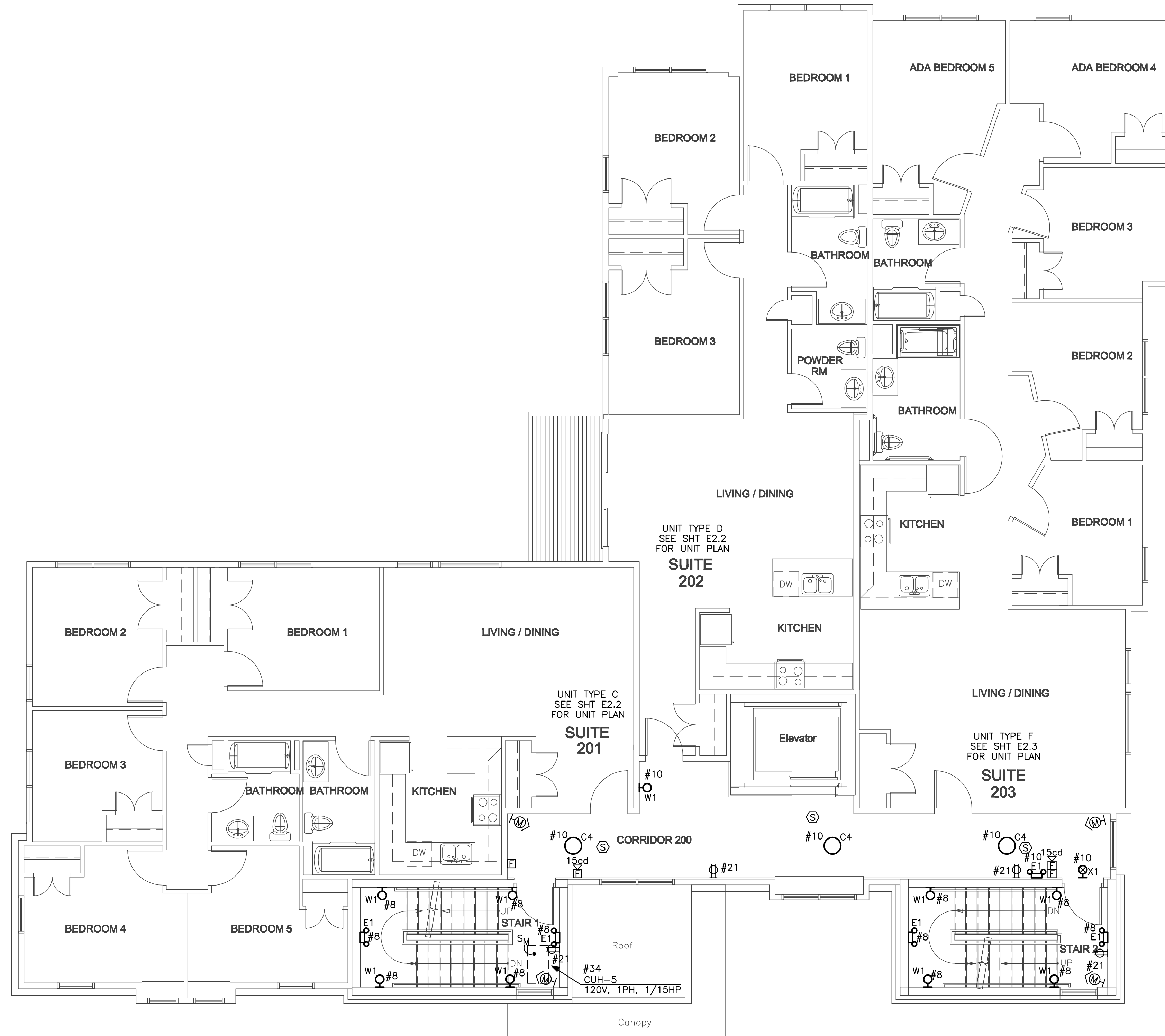
SECOND FLOOR PLAN 3/16" = 1'-0"
