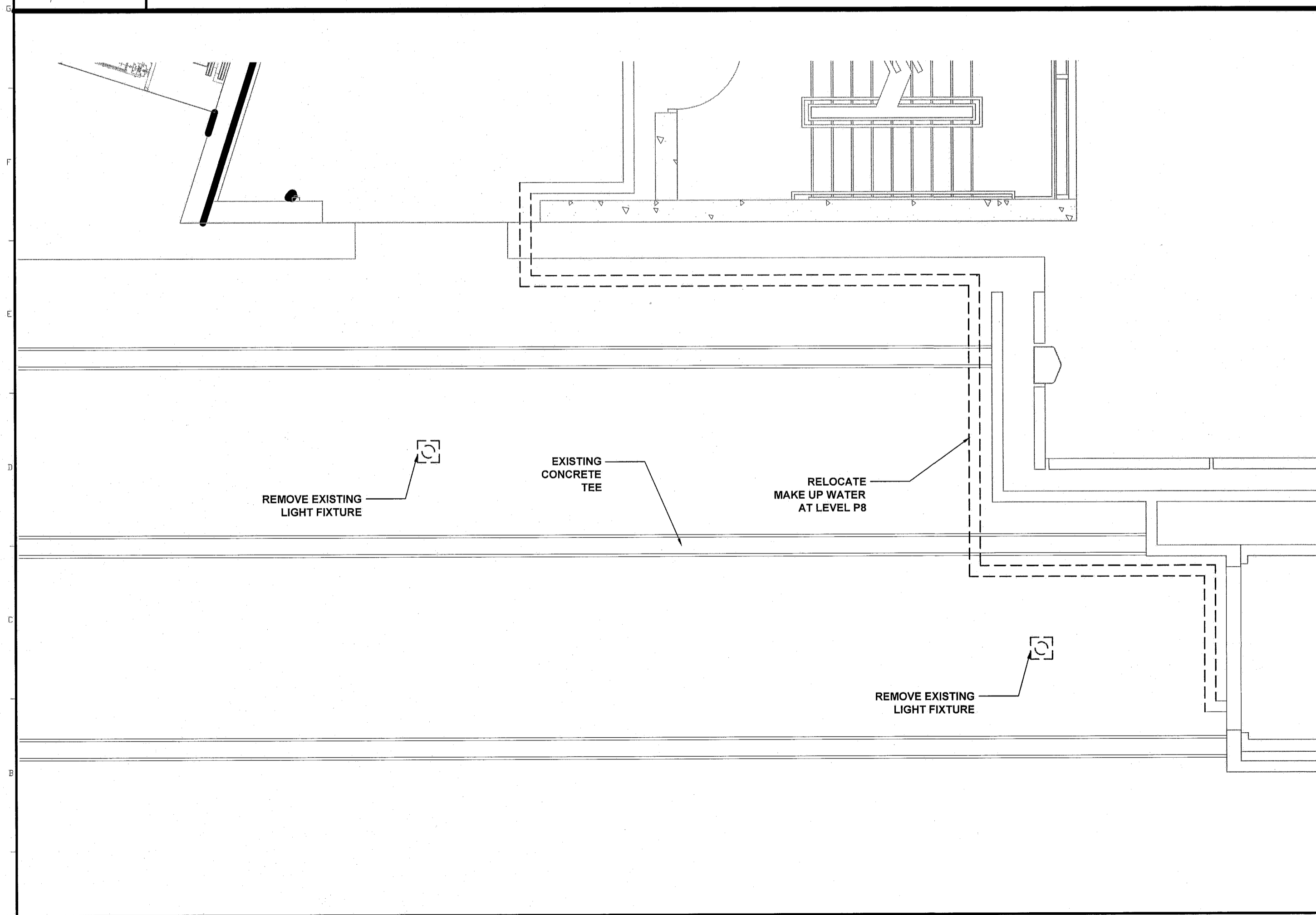
A1 REFLECTED CEILING REMOVALS PLAN LEVEL 8
