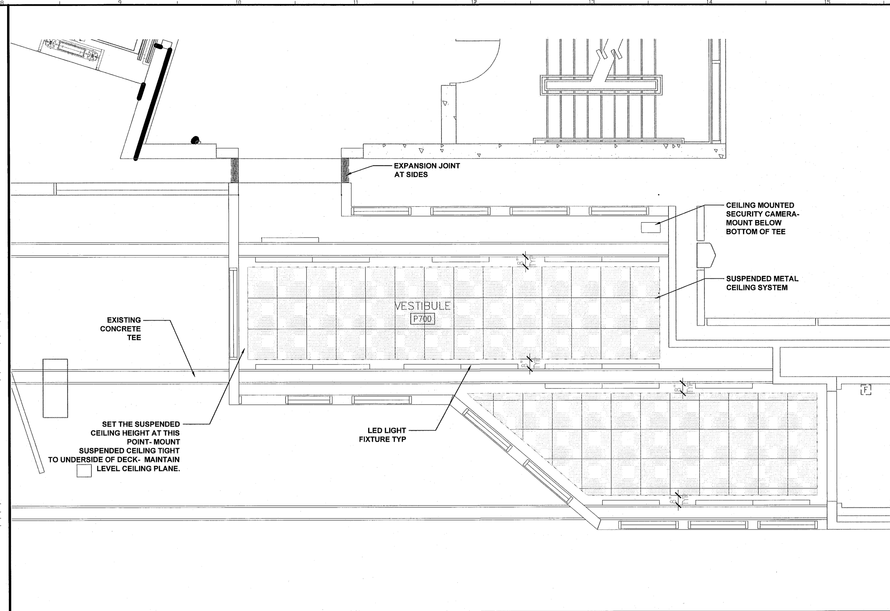
E7 REFLECTED CEILING PLAN LEVEL 7
