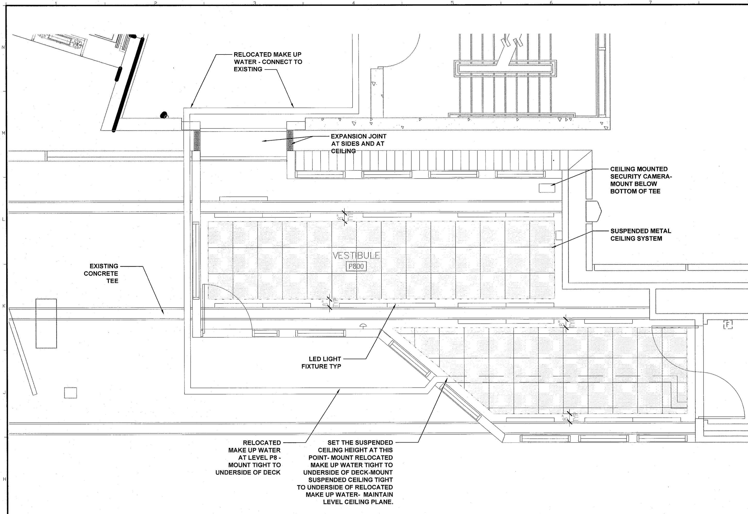
E1 REFLECTED CEILING PLAN LEVEL 8
