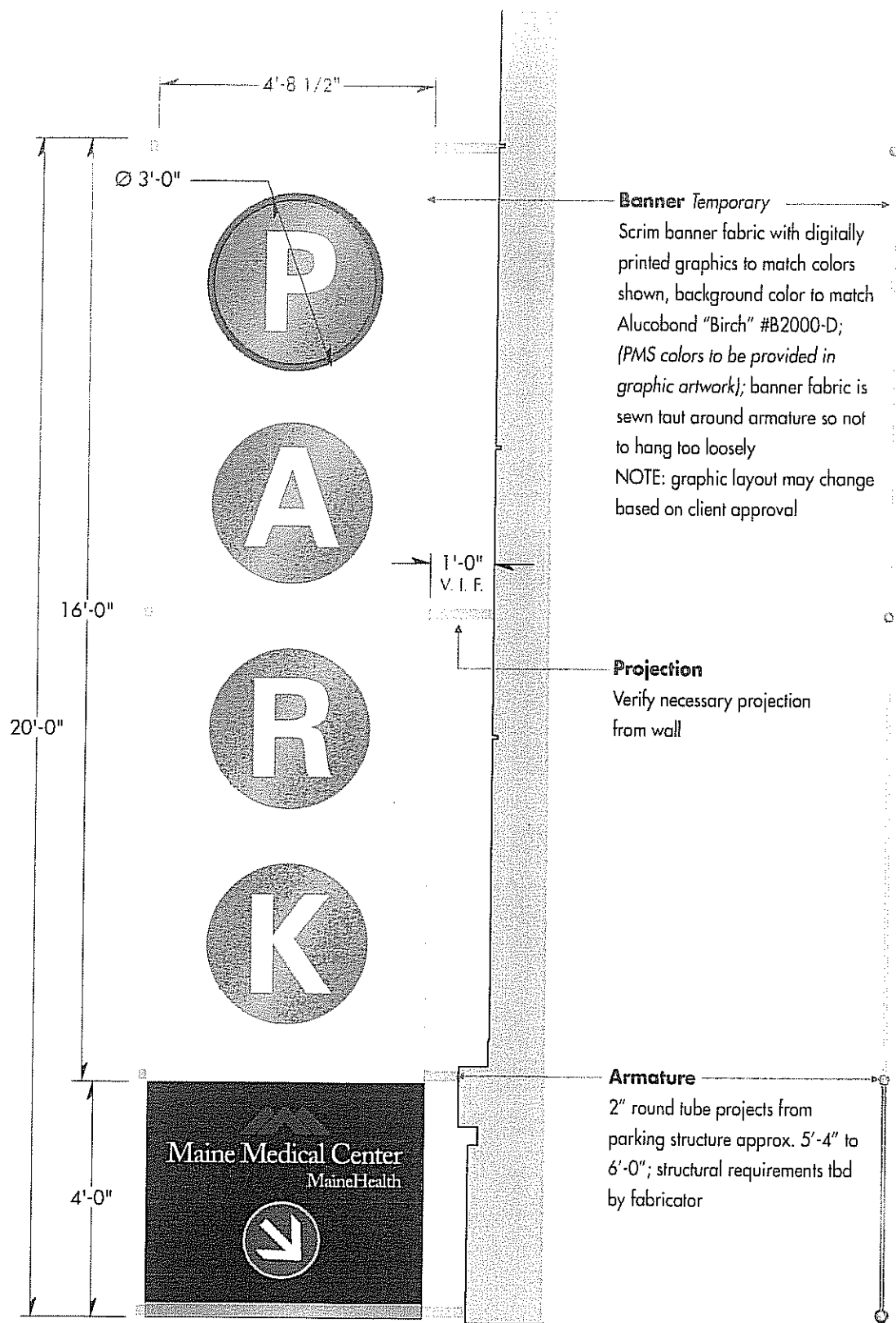
A Temporary Parking Banner Side Elevation Scale: 3/8" = 1'-0"
