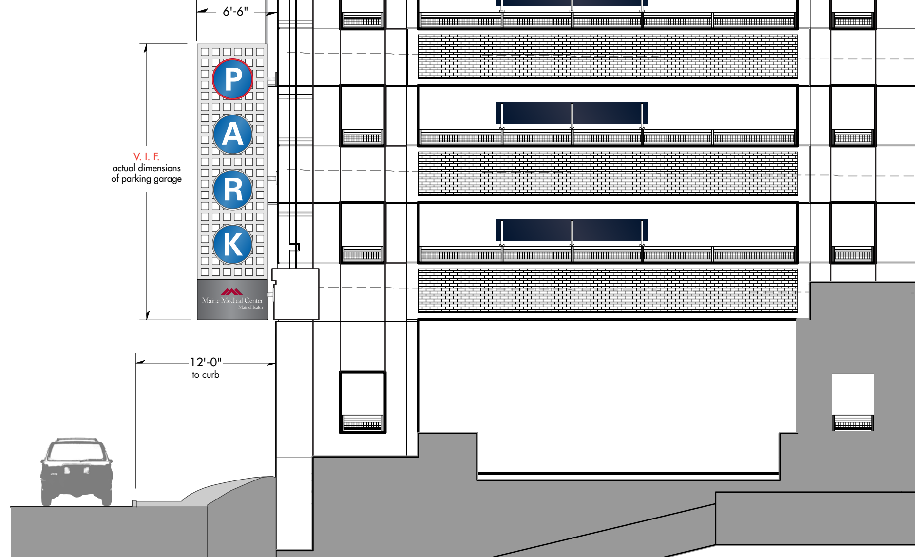
PID 1A Projecting Parking Entry ID view up Congress Street illuminated/dimensional Scale: 1/8" = 1'-0"
