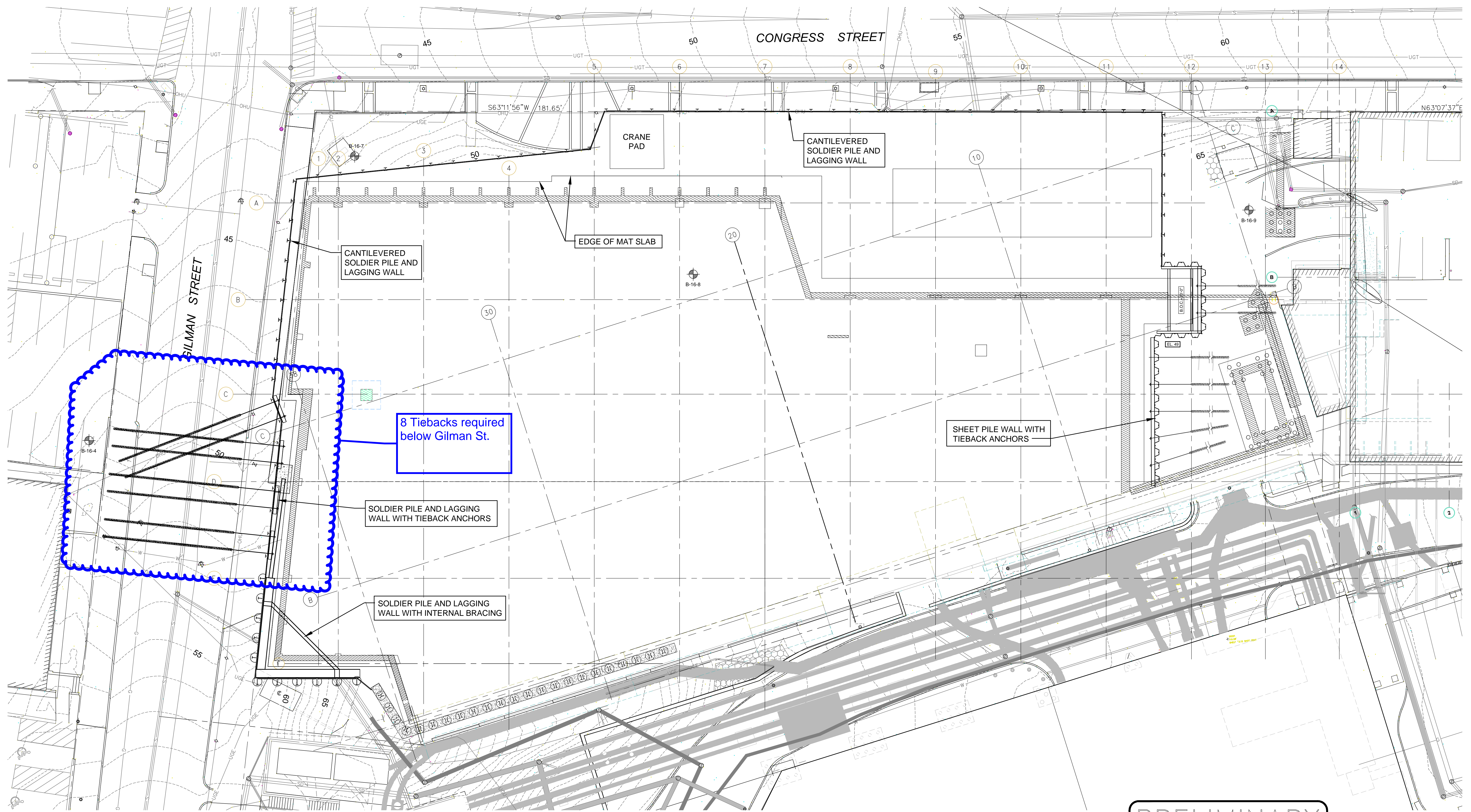
PLAN OF EXCAVATION SUPPORT SCALE: 1"=15'-0"
