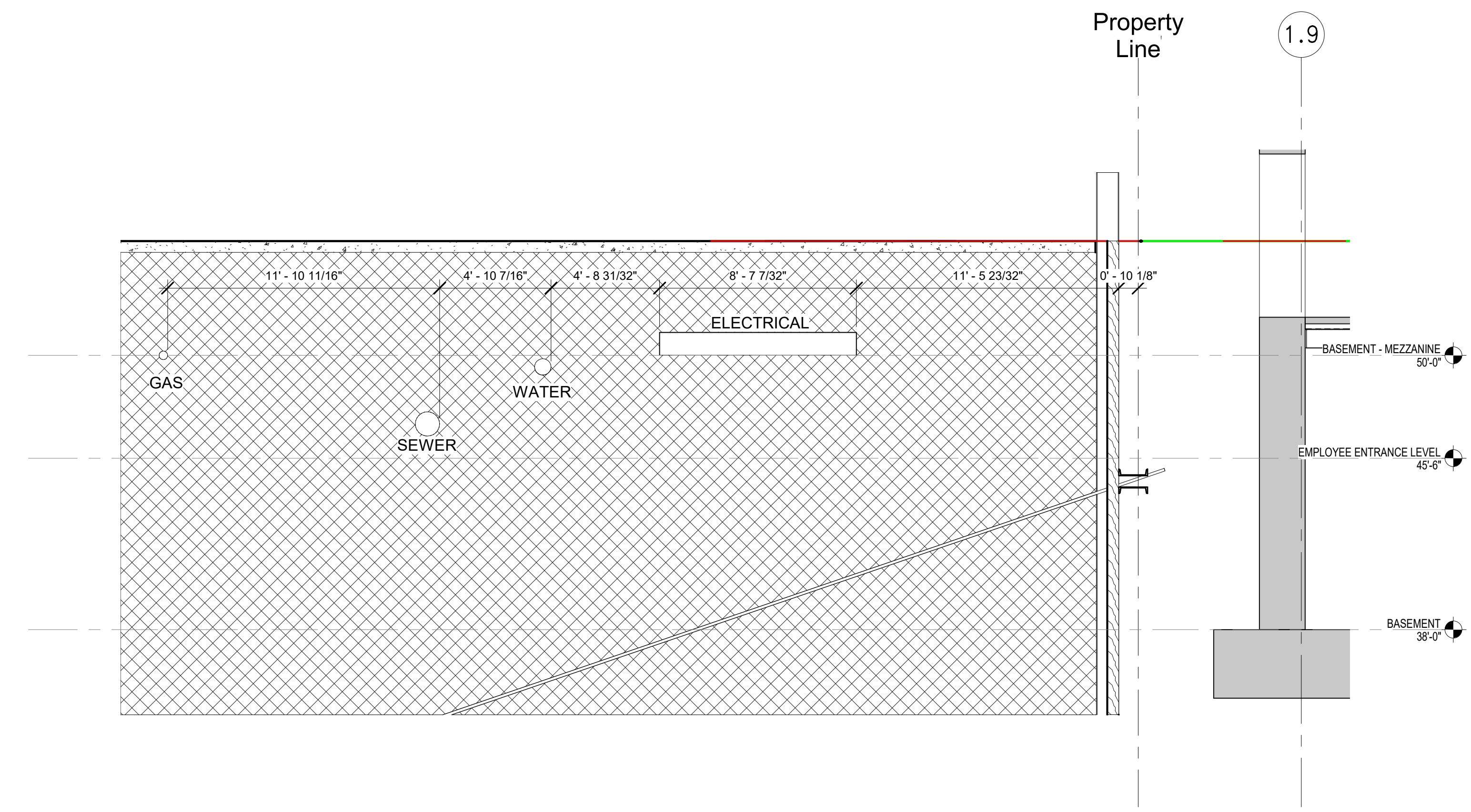
3 Section 2 1/4" = 1'-0"
