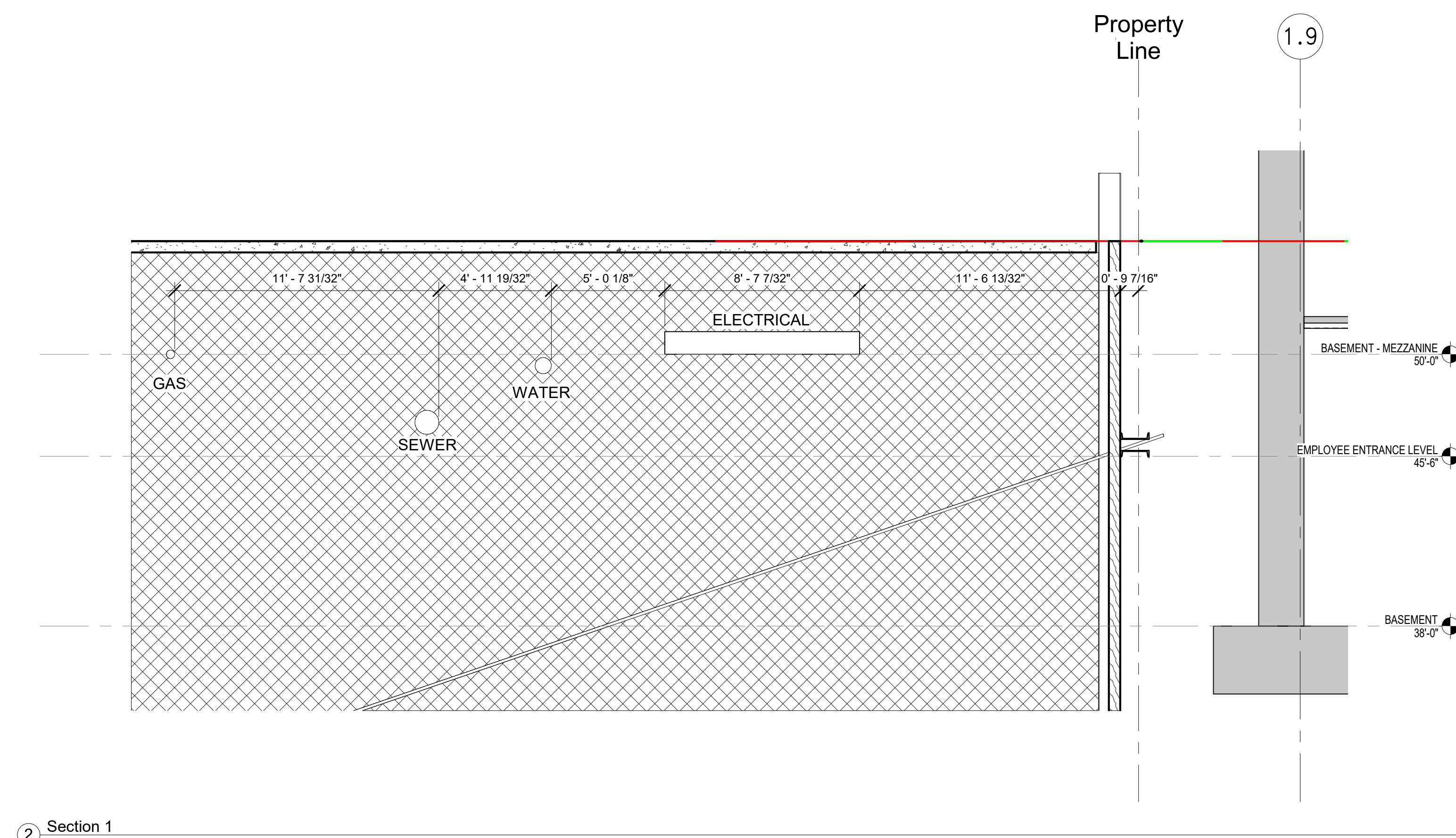
2 Section 1 1/4" = 1'-0"
