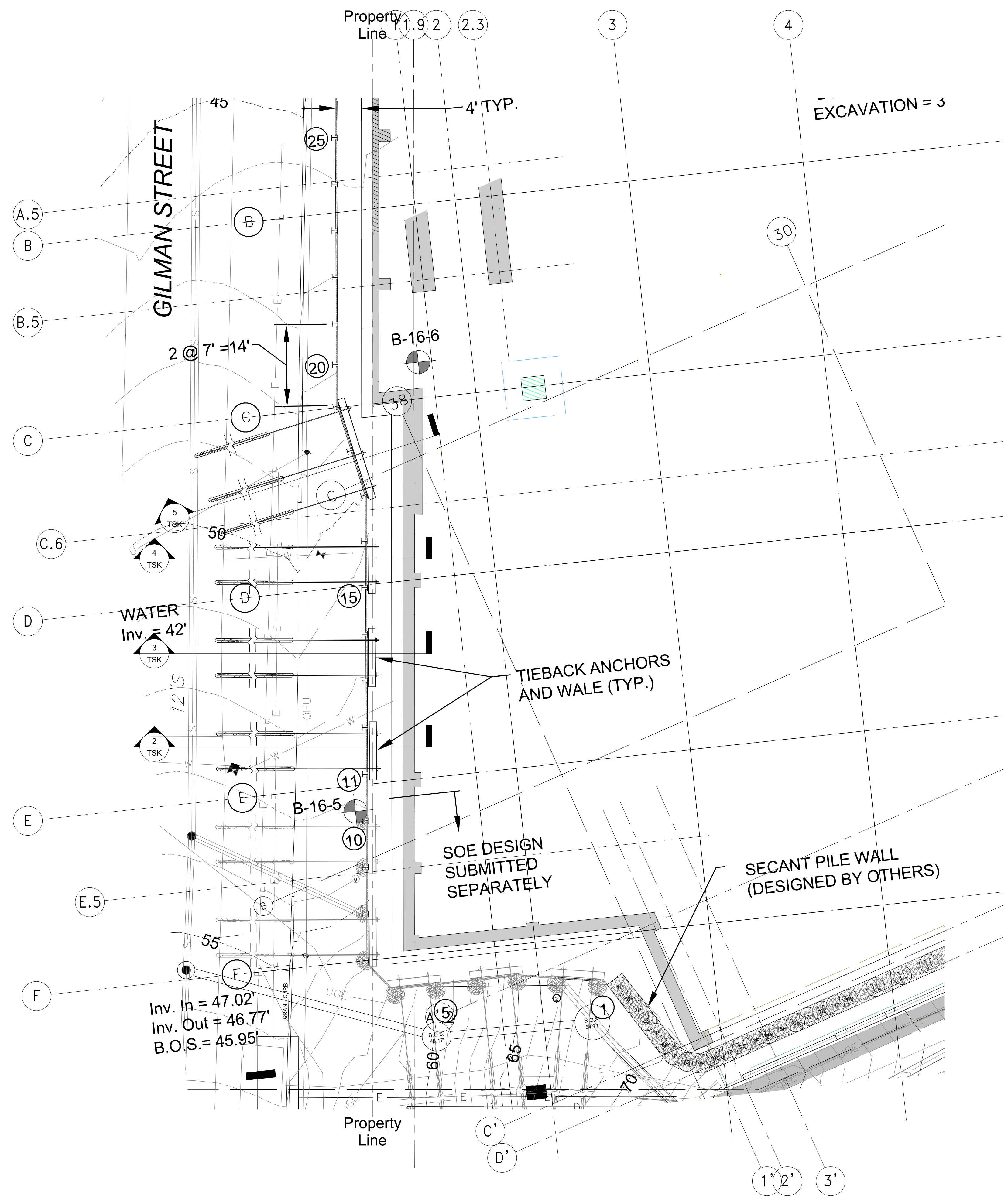
1 Site 1" = 10'-0"
