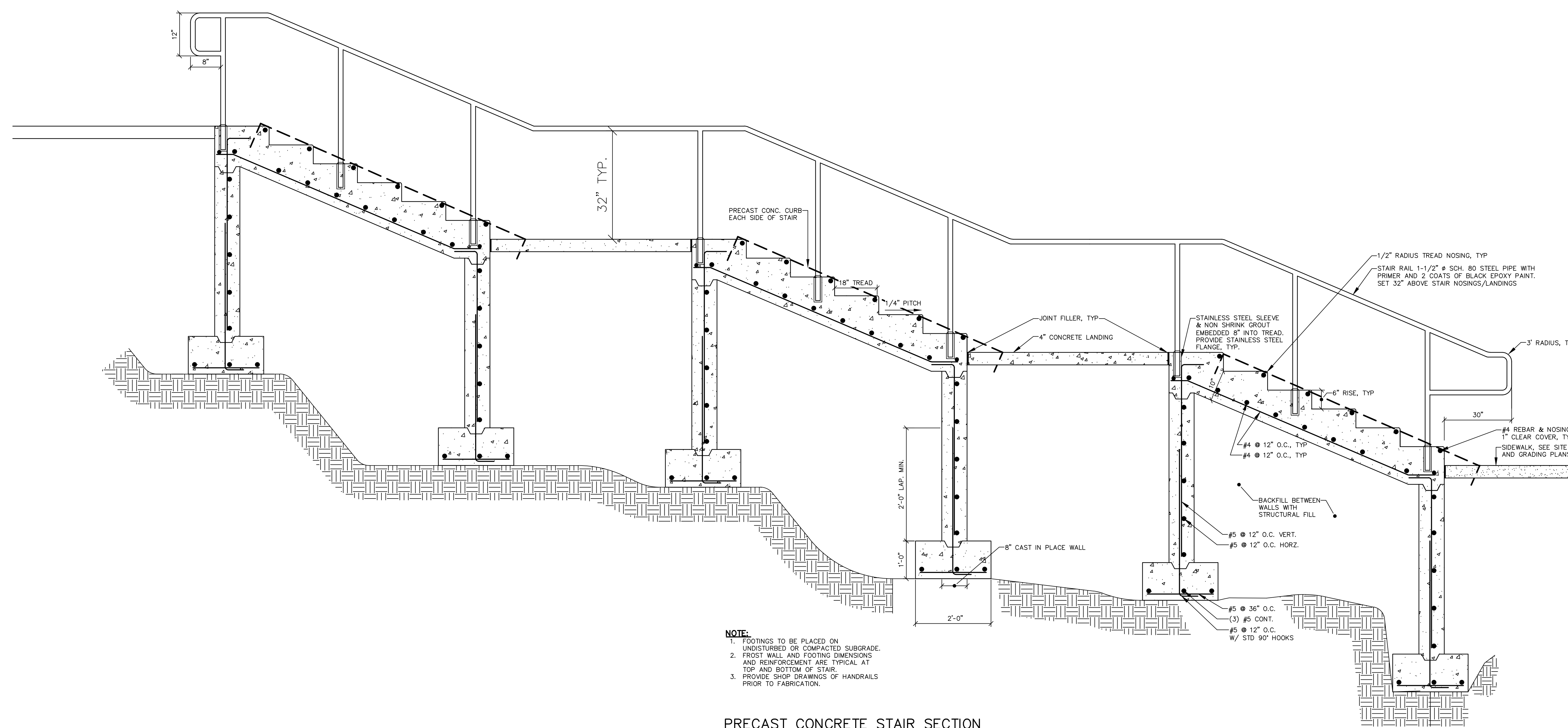
PRECAST CONCRETE STAIR SECTION NOT TO SCALE
